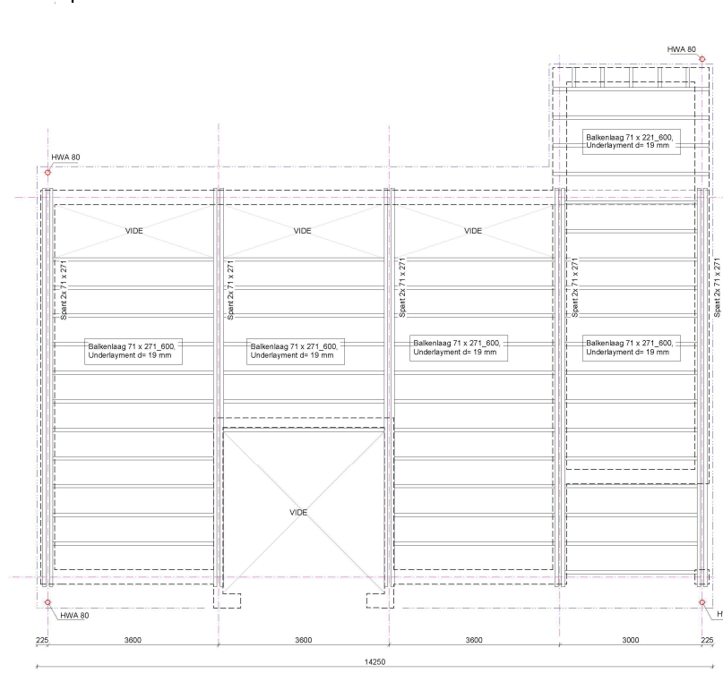
Dakplan
