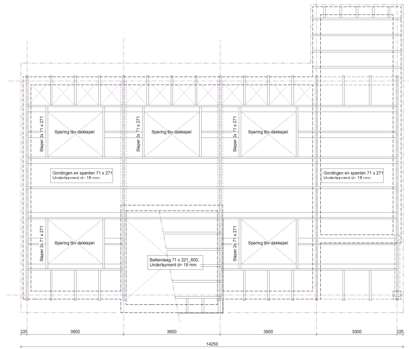
Dakplan
