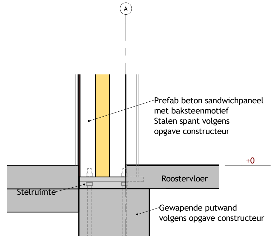
Detail 2 1:10
