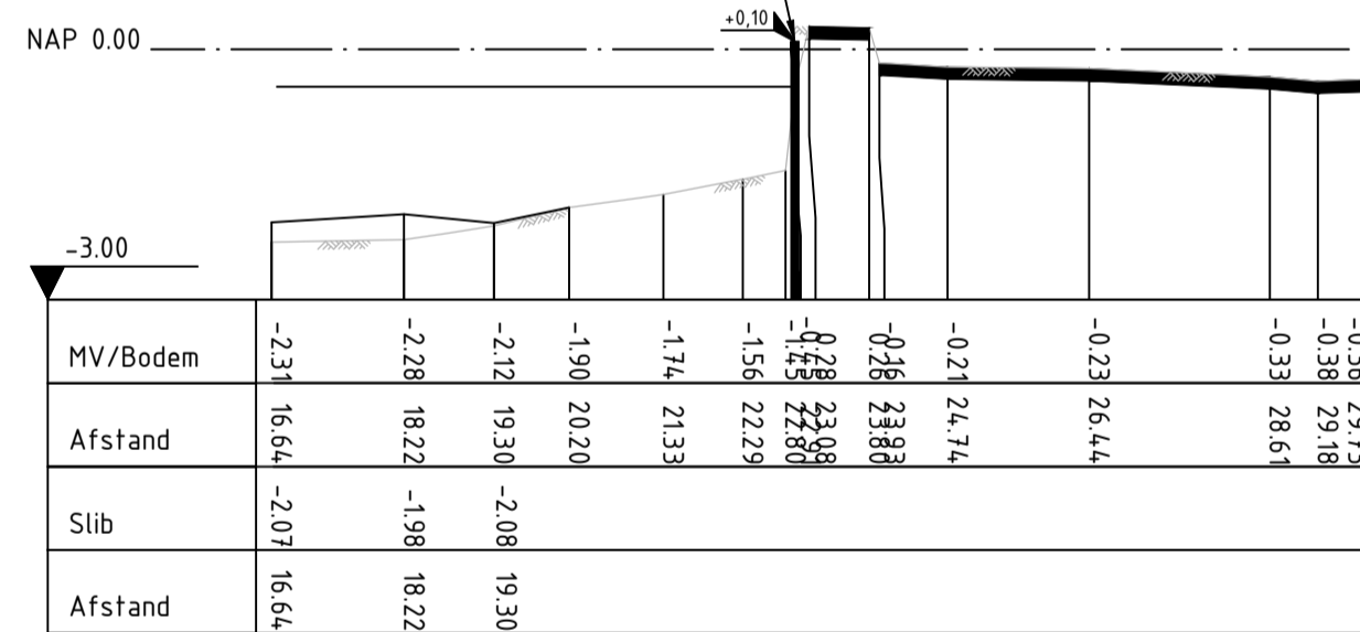
DWP 03 Kadevak RK111-470 (1) Schaal 1:100
