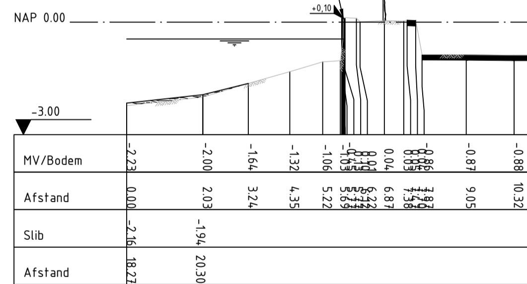
DWP 04 Kadevak RK111-470 (2) Schaal 1:100
