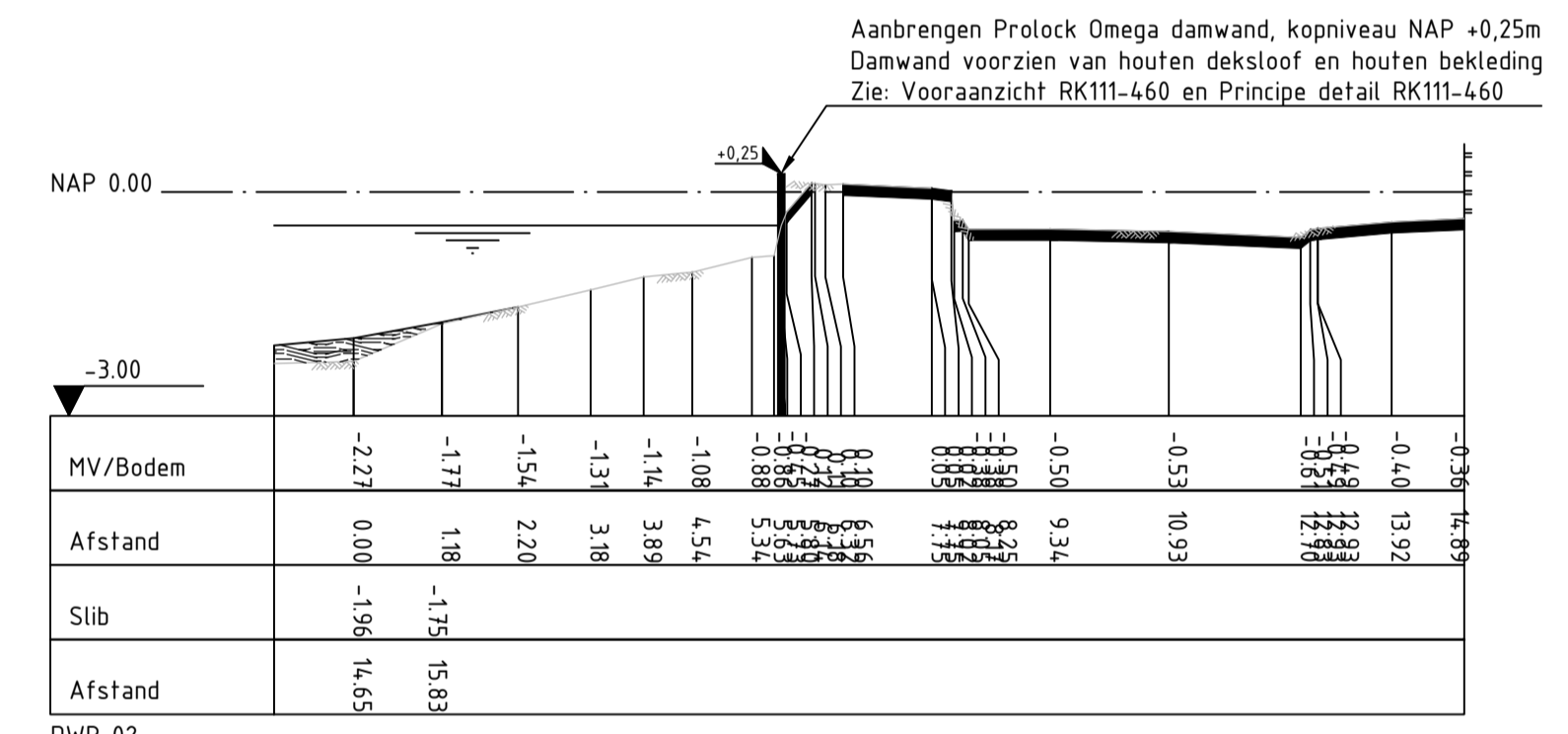
DWP 02 Kadevak RK111-460 Schaal 1:100
