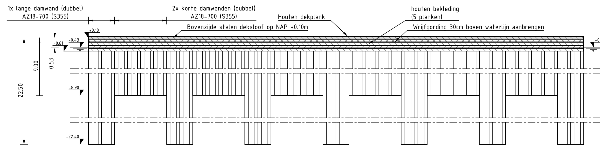
DWP 04 Kadevak RK111-470 (2) Schaal 1:100
