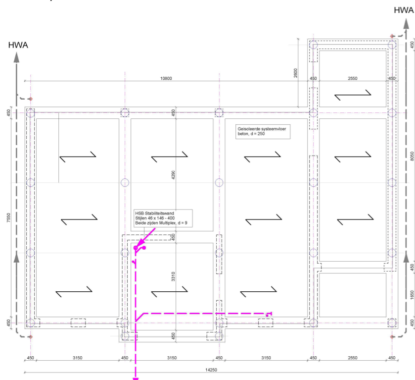
Fundering - riolering
