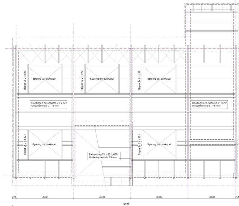
Dakplan
