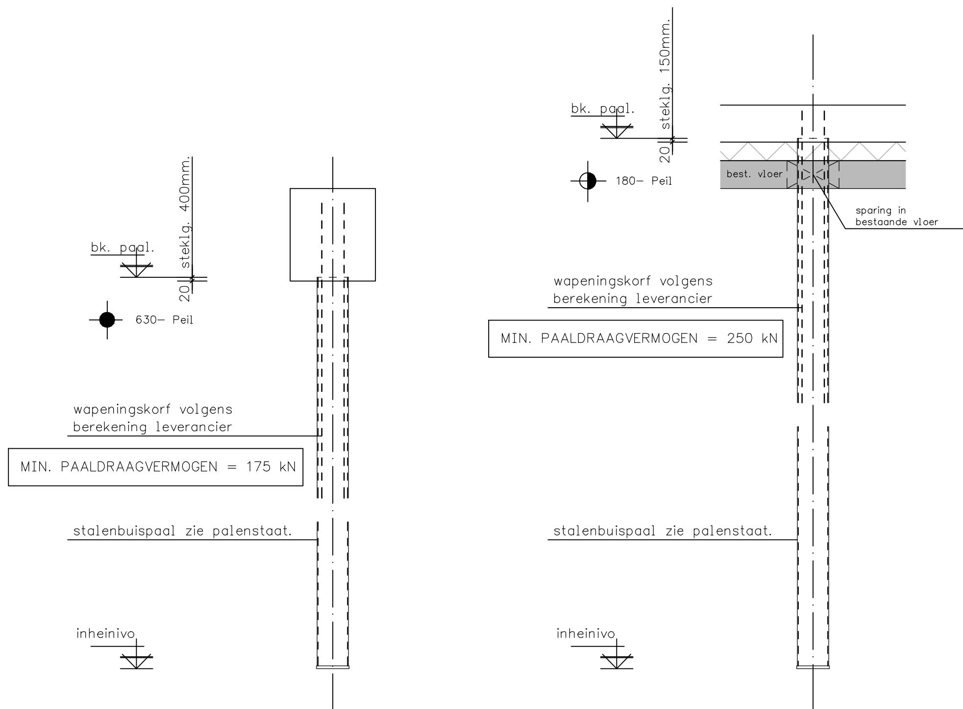
PAALDETAILS.
