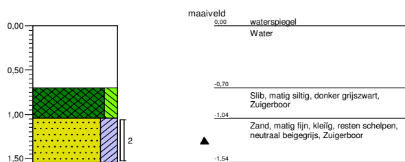
Boring: 1014
