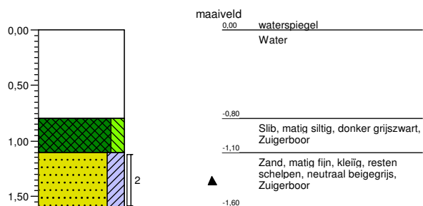
Boring: 1007
