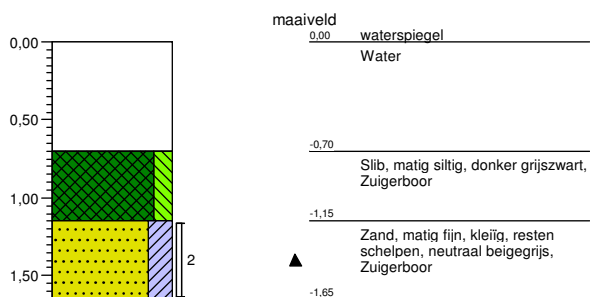
Boring: 1006
