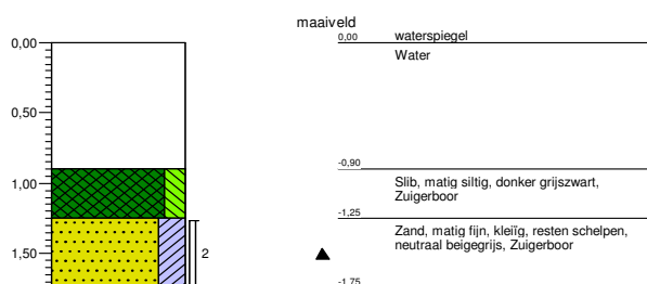
Boring: 1019
