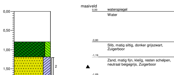
Boring: 1016
