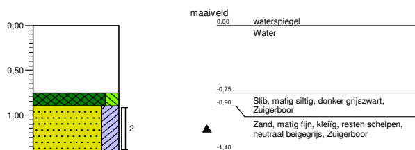
Boring: 1011
