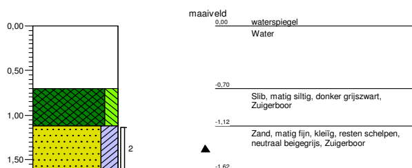
Boring: 1013
