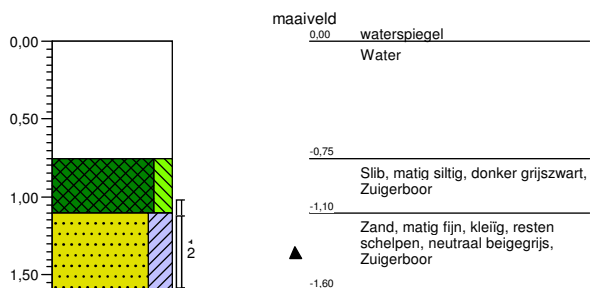
Boring: 1010
