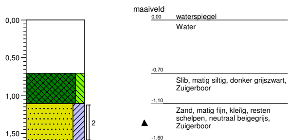
Boring: 1009
