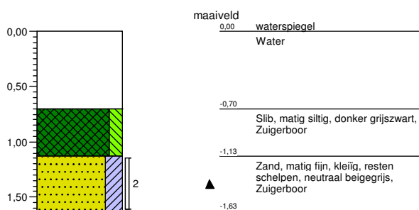
Boring: 1010
