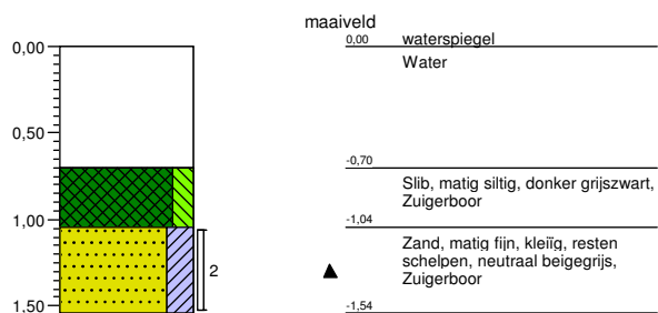
Boring: 1005
