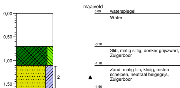
Boring: 1009
