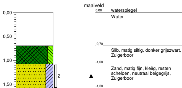
Boring: 1004
