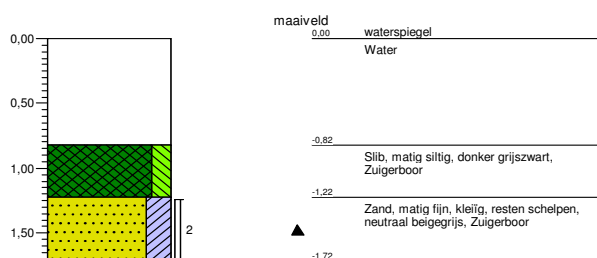
Boring: 1015
