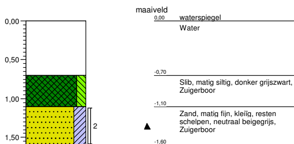
Boring: 1008
