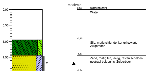
Boring: 1020
