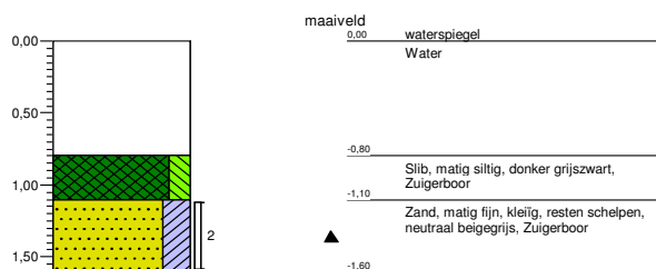
Boring: 1012
