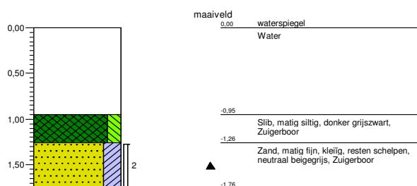
Boring: 1020
