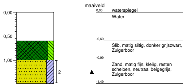
Boring: 1003
