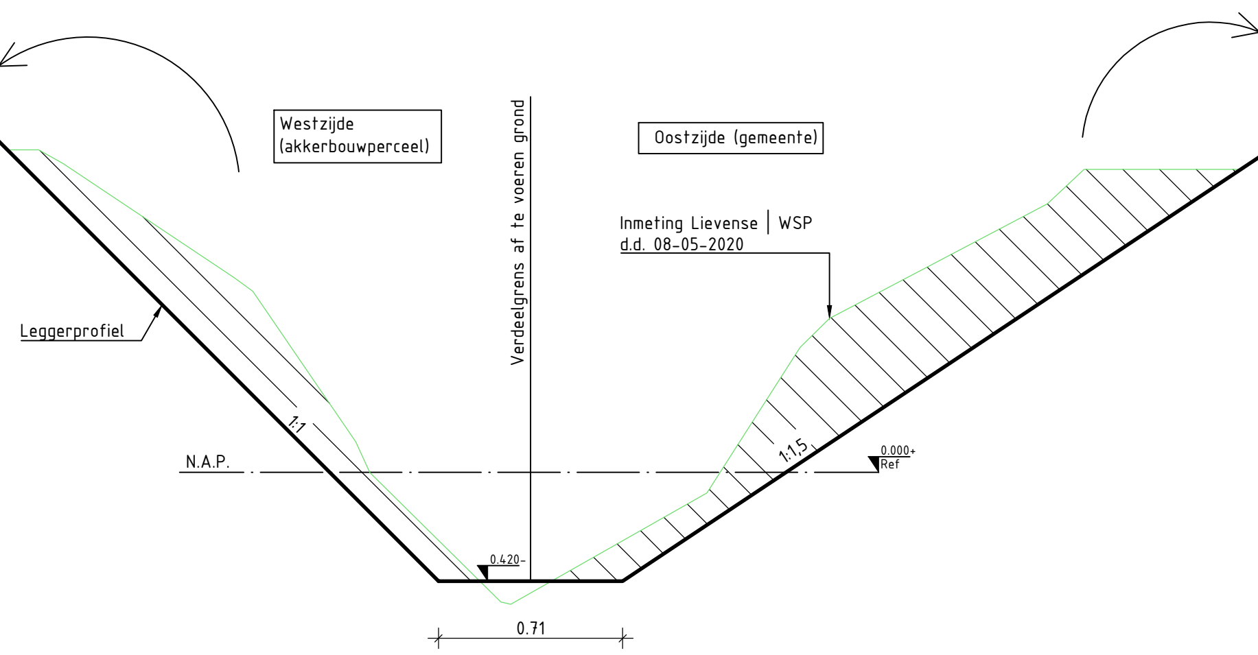
PRINCIPEDOORSNEDE LEGGER WATERGANG SCHAAL 1:20
