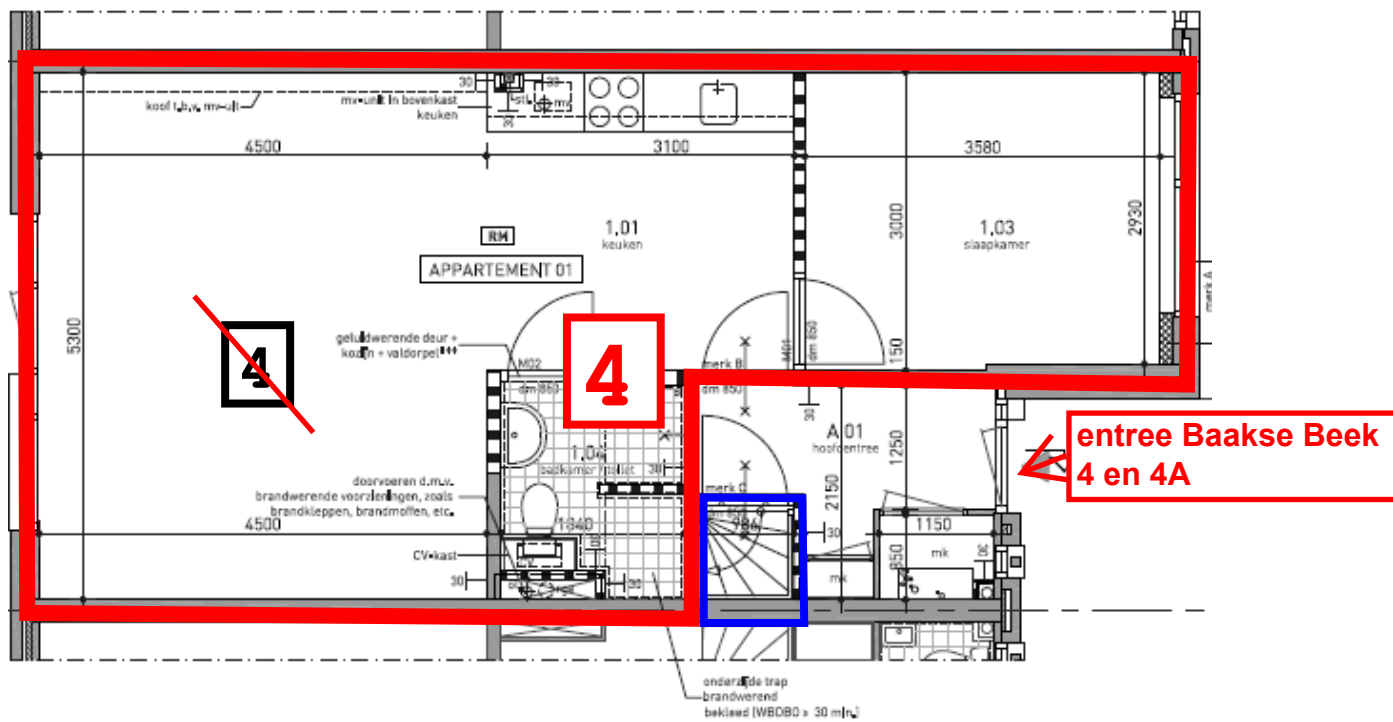
begane grond (0.000+)
