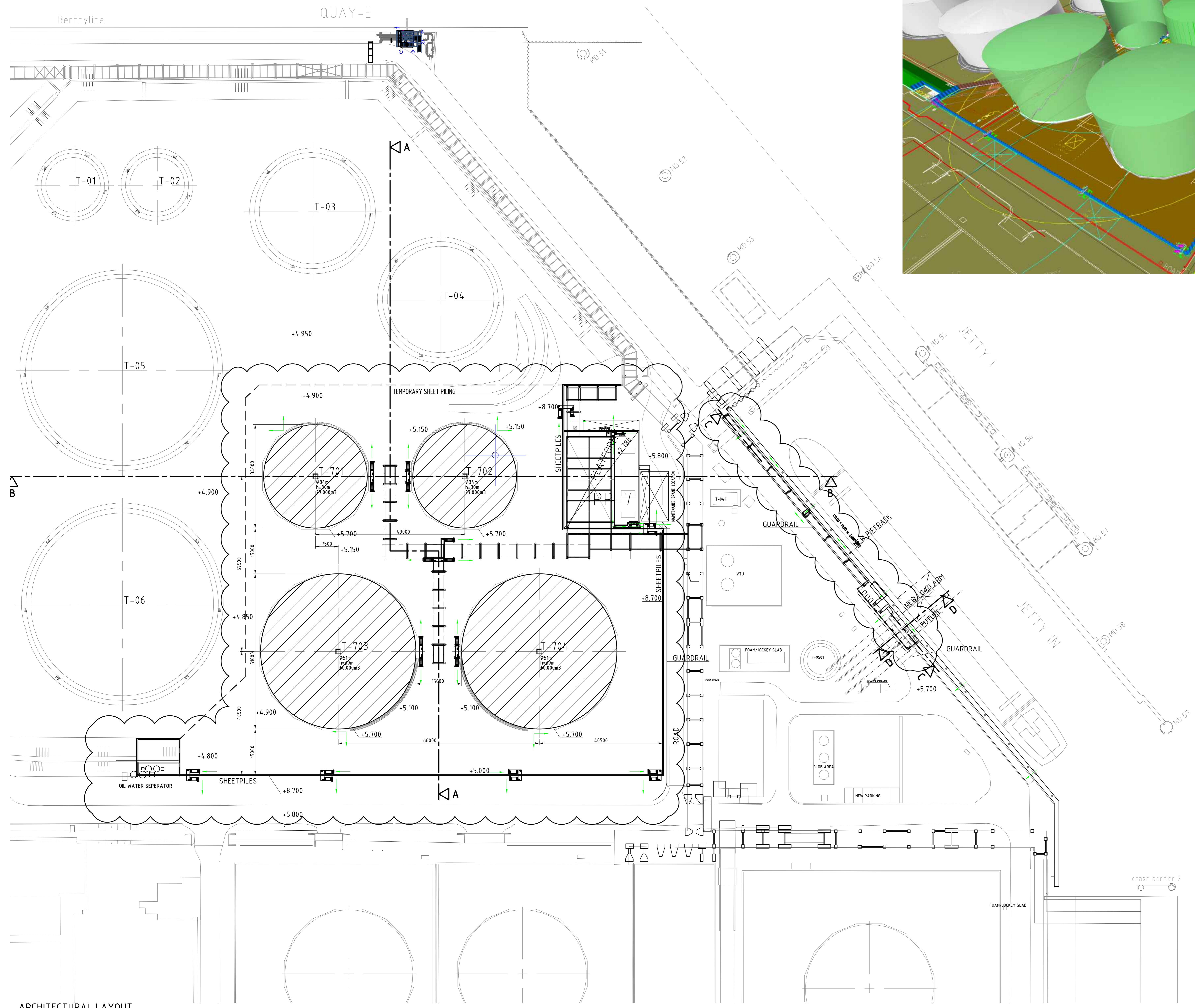
ARCHITECTURAL LAYOUT SCALE 1:500
