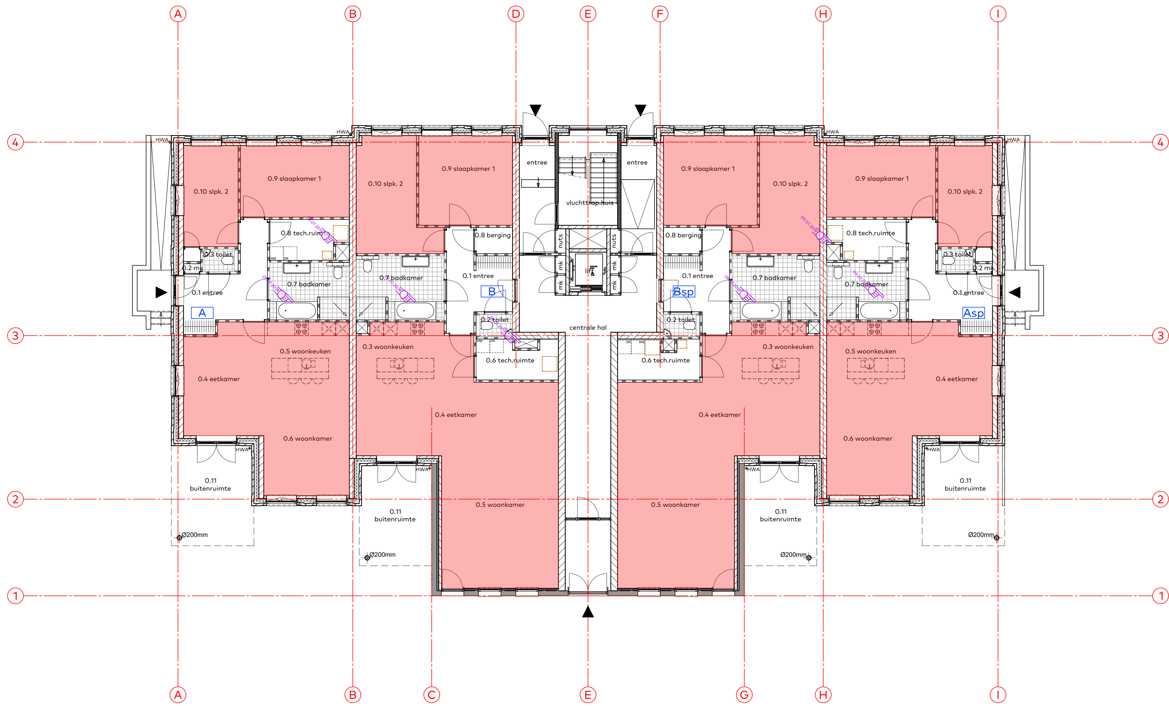
Begane grond VG appartement A = 71,5 m 2 VG appartement B = 103,0 m 2
