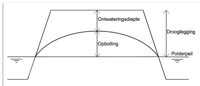
Figuur 6: Drooglegging.
