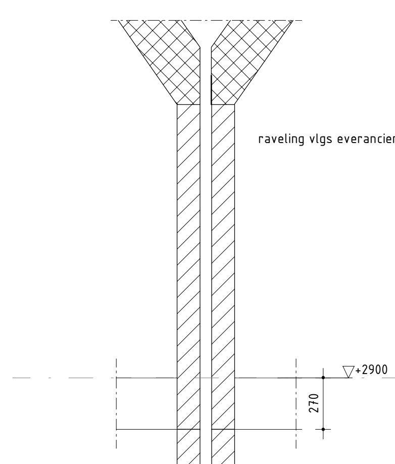
Detail 1.05 1: 20
