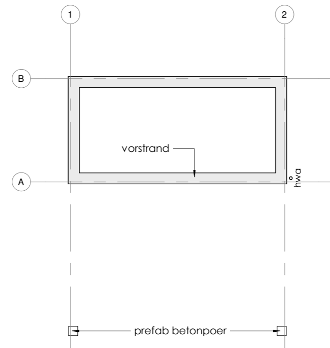
FUNDERING
