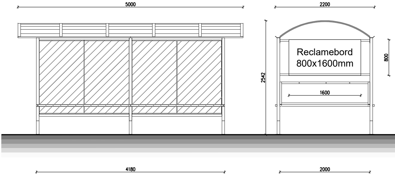
ZB-stalling schaal 1:50
