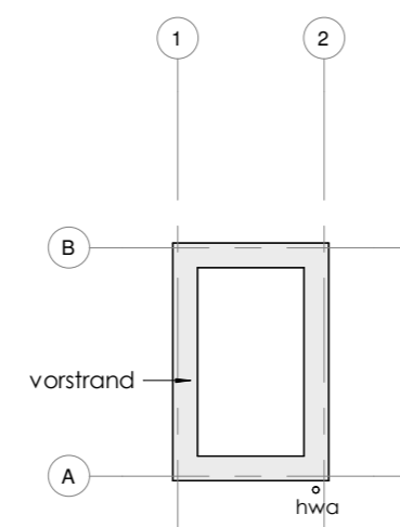
FUNDERING
