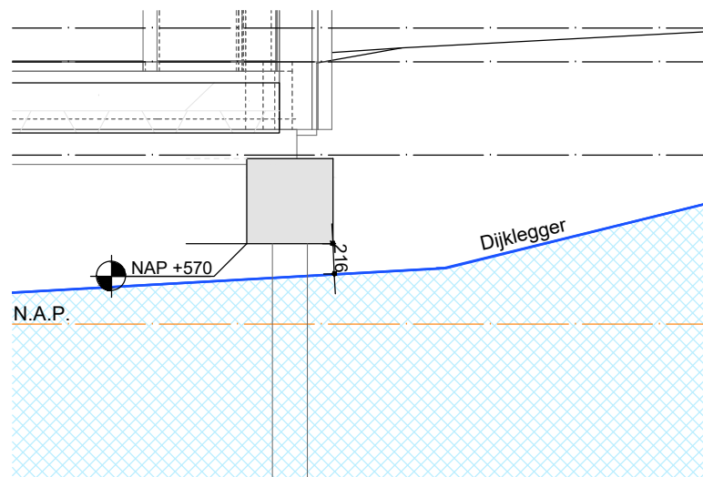
DETAIL 4A 1:50
