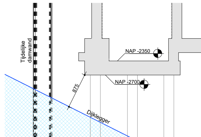
DETAIL 4B 1:50
