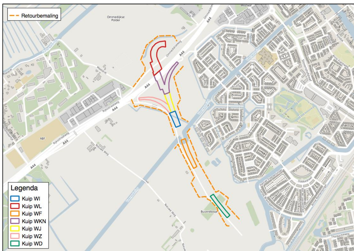
Figuur 10: Locaties retourbemaling.
