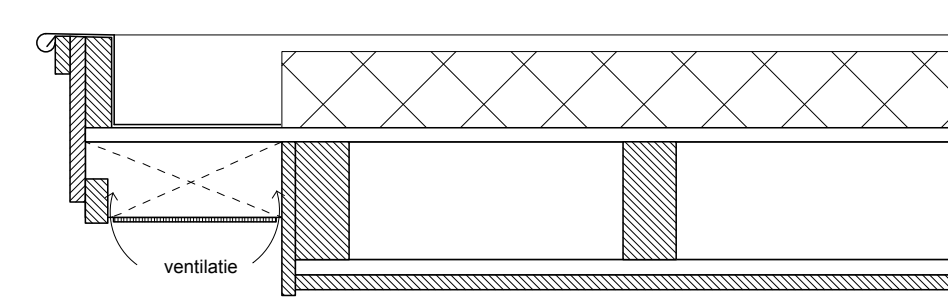
dakranddetail overstek luifel
