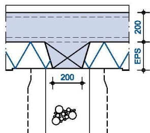
DETAIL 4 - RAVEELOPLEGGING
