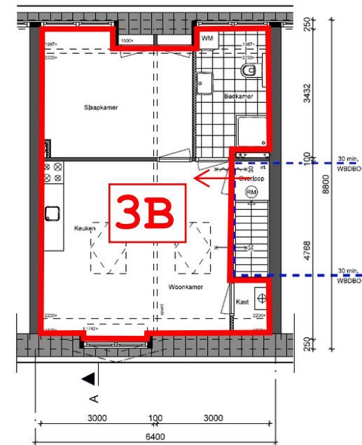
Zolder (appartement 3)
