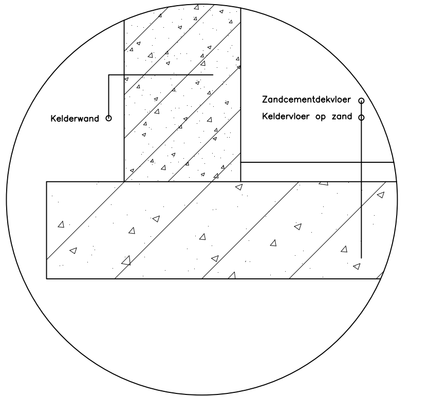
Details 1:10
