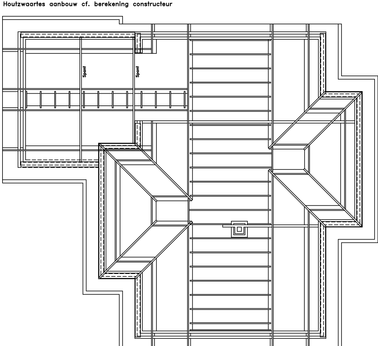
Zolderbalklaag
