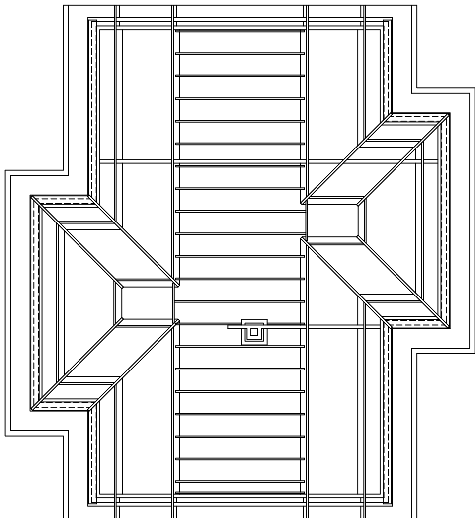
Zolderbalklaag
