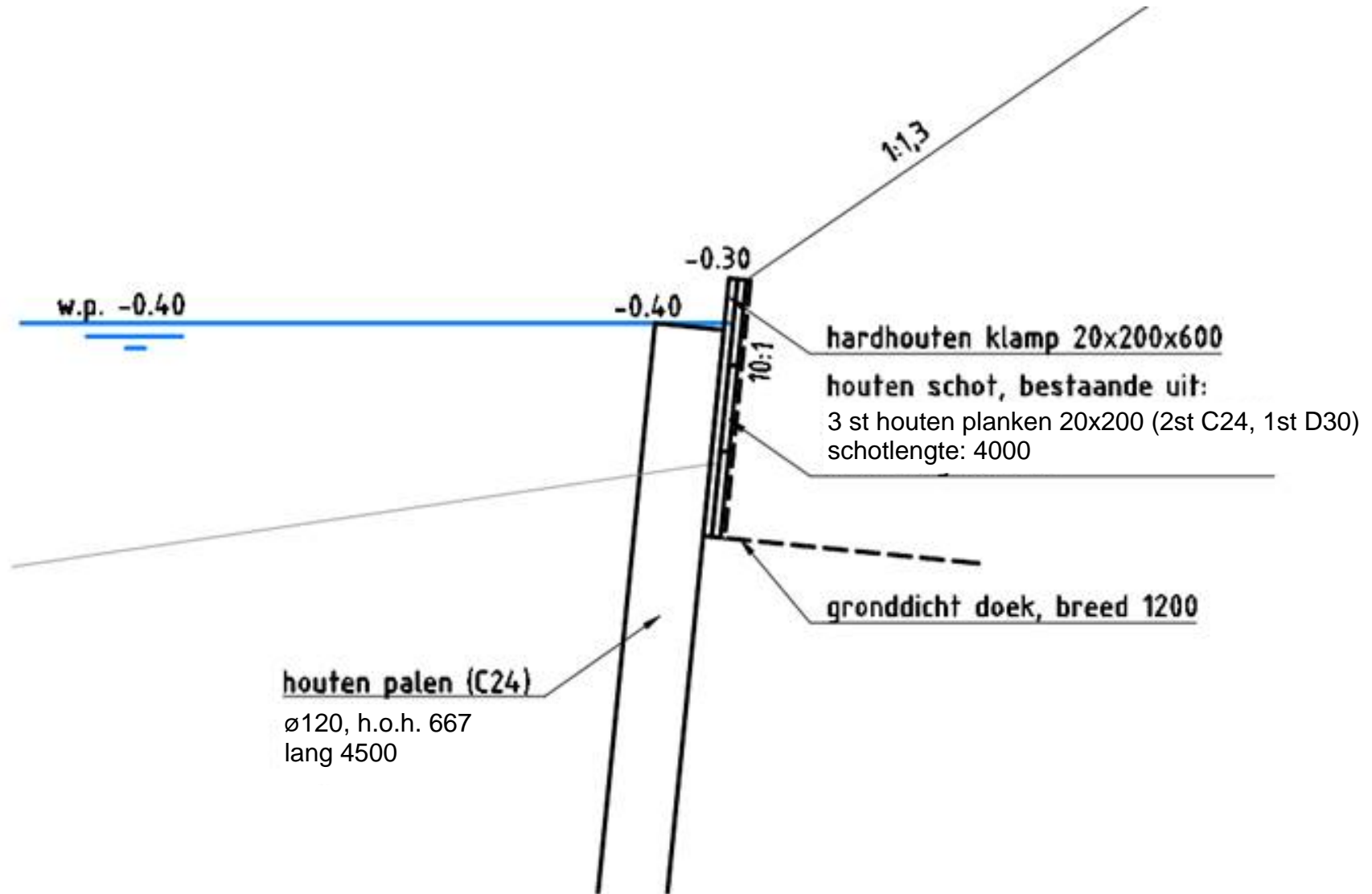
Principedetail beschoeiing
