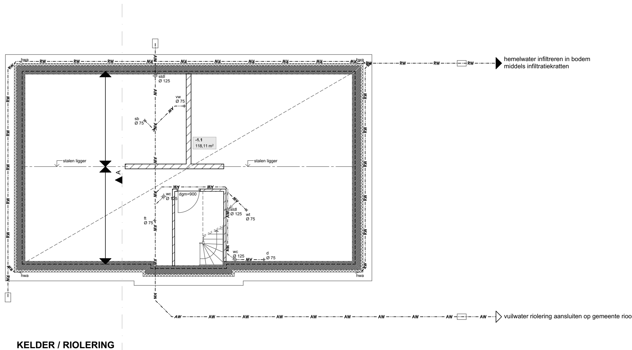
KELDER / RIOLERING
