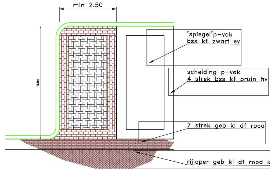
Detail parkeervak 1: conform HIBOR (I)
