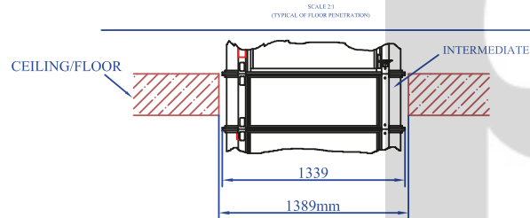
DETAIL "A" SCALE 2:1 (TYPICAL OF FLOOR PENETRATIONS)
