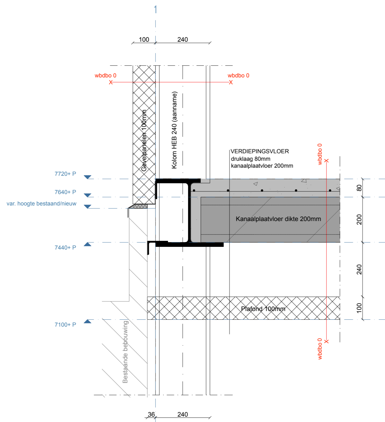
DETAIL 14
