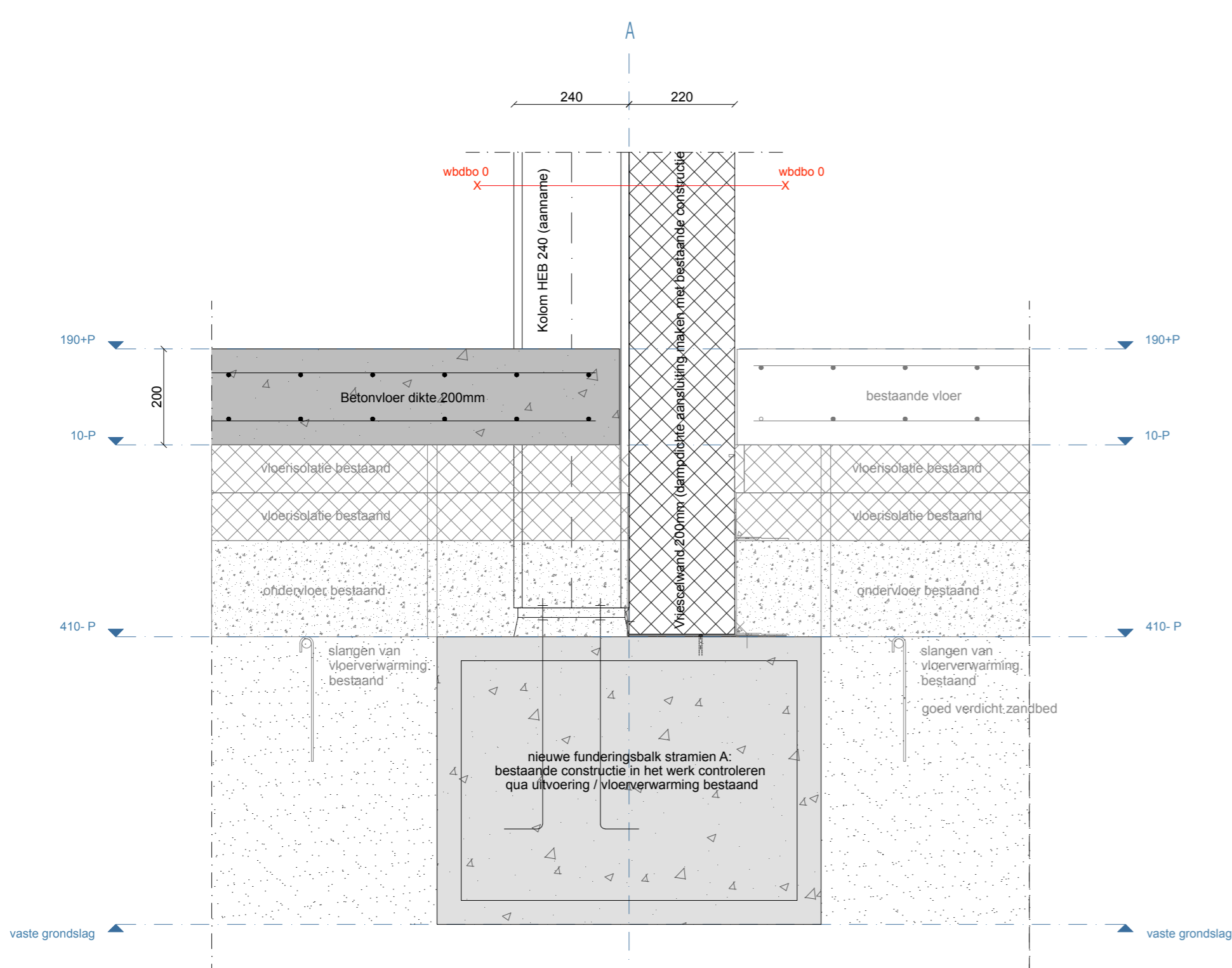
DETAIL 15
