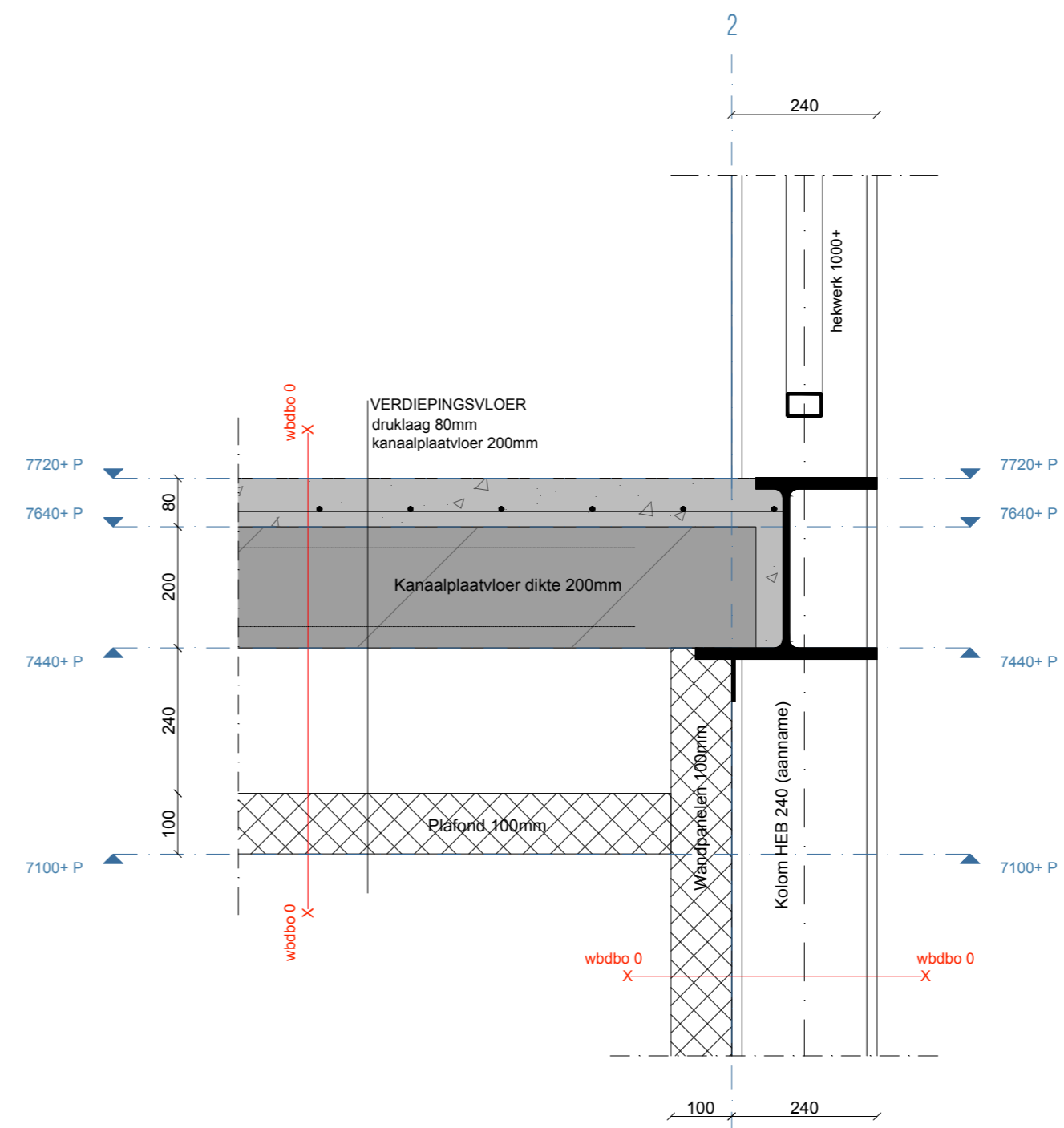
DETAIL 17
