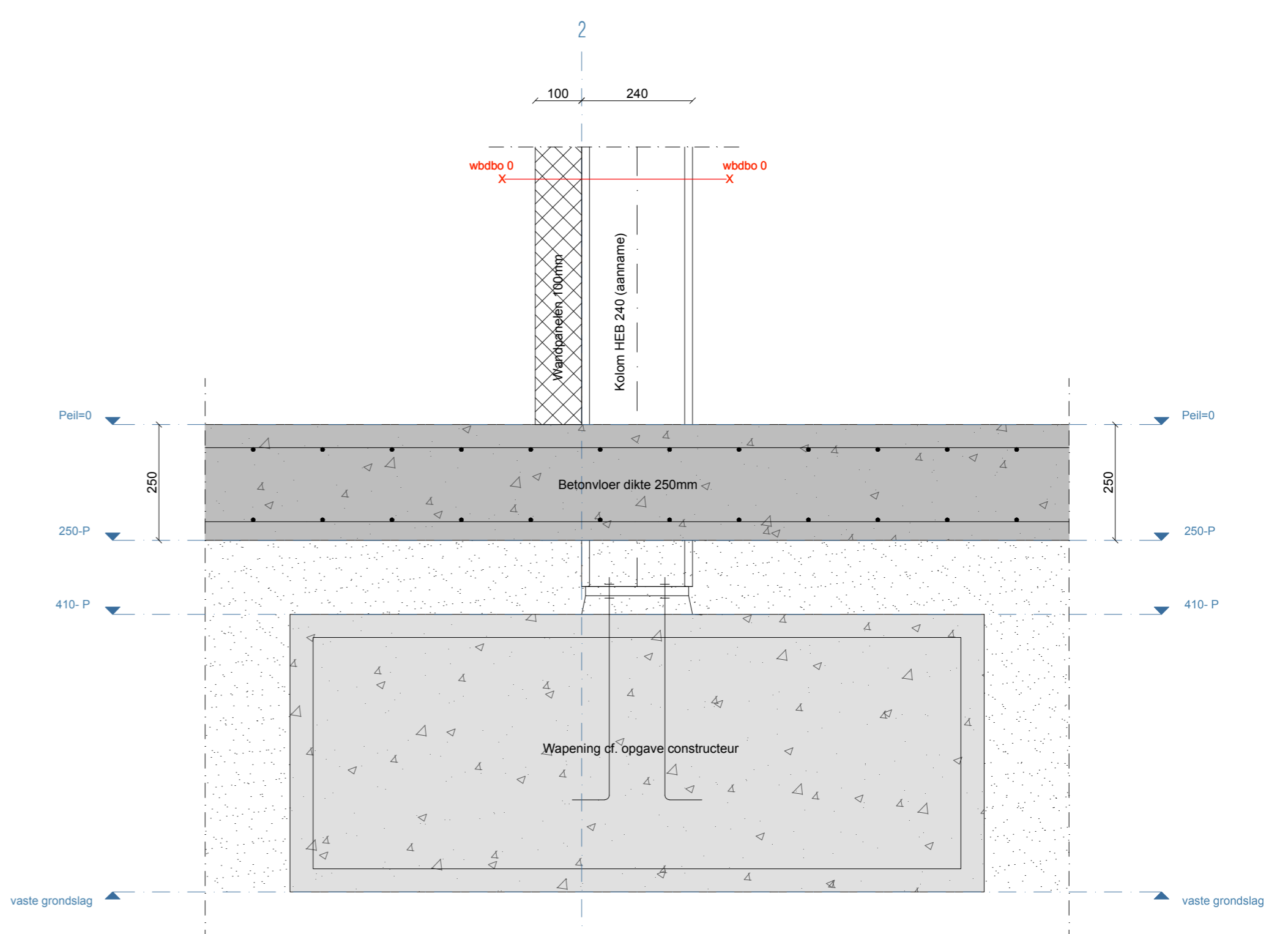
DETAIL 18
