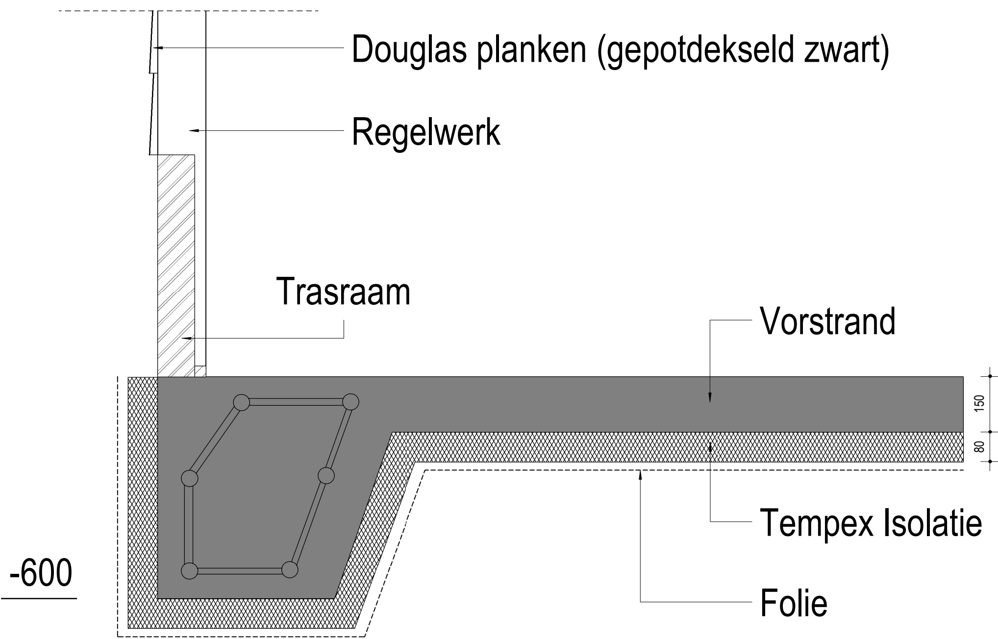
Detail fundering 1:10
