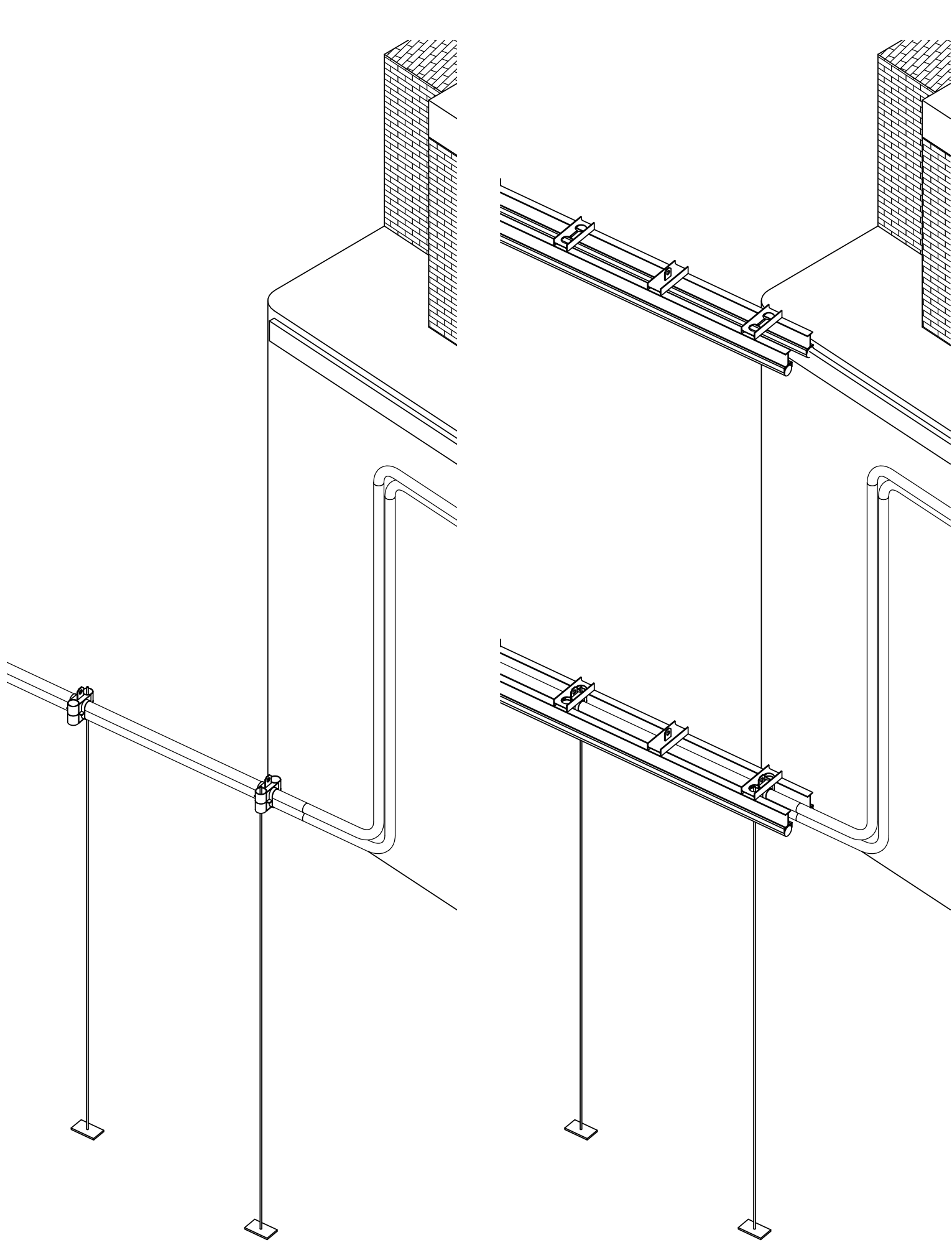
3D DETAIL ZINKER
