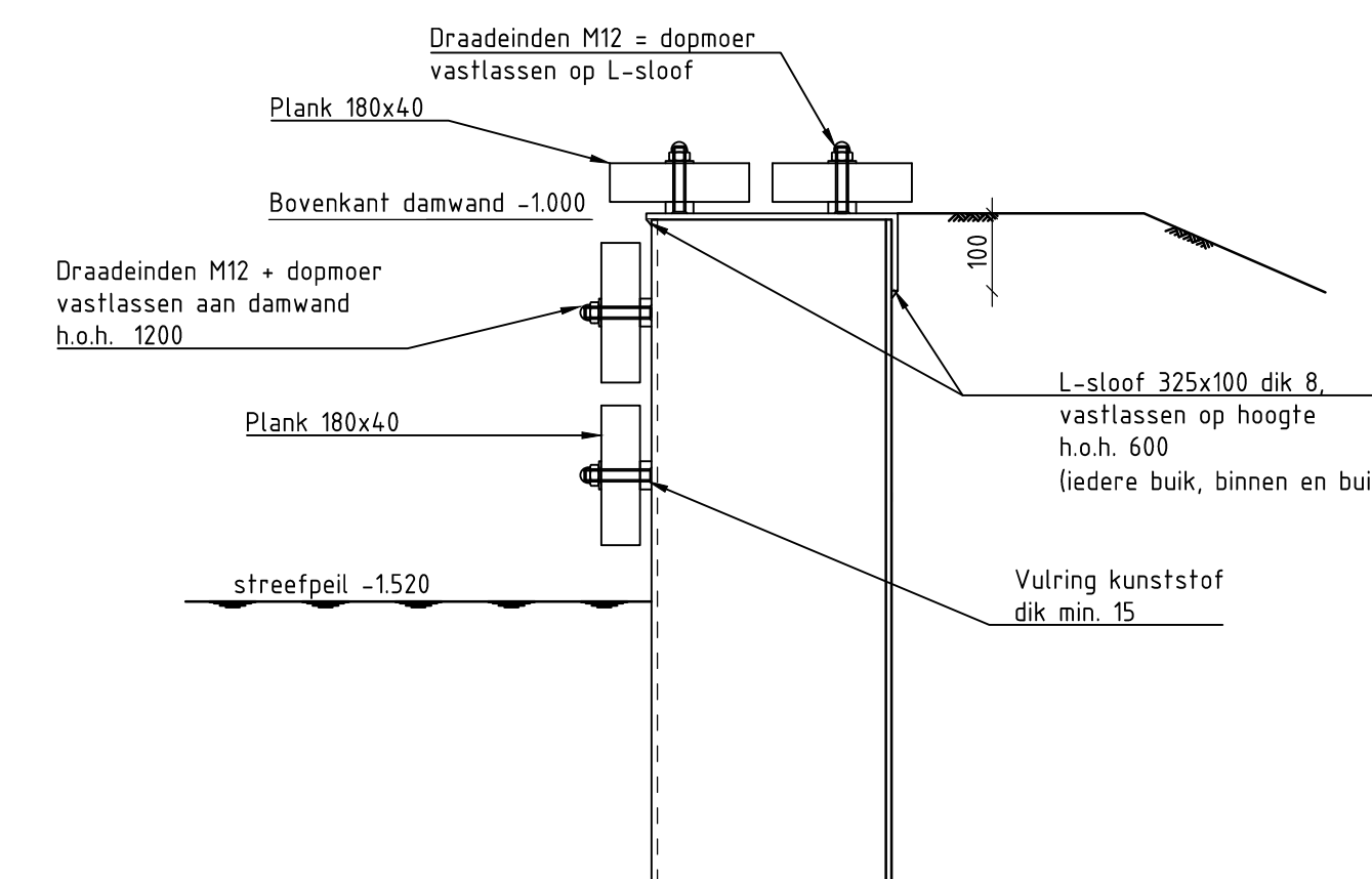
Detail lambrisering SCHAAL 1:10
