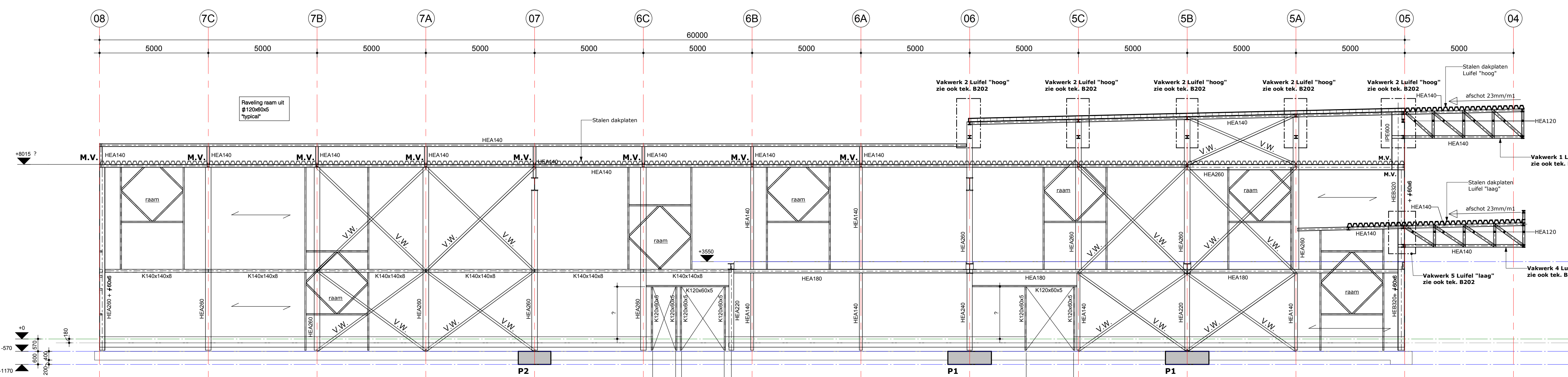
Drsn in as G 1 : 100
