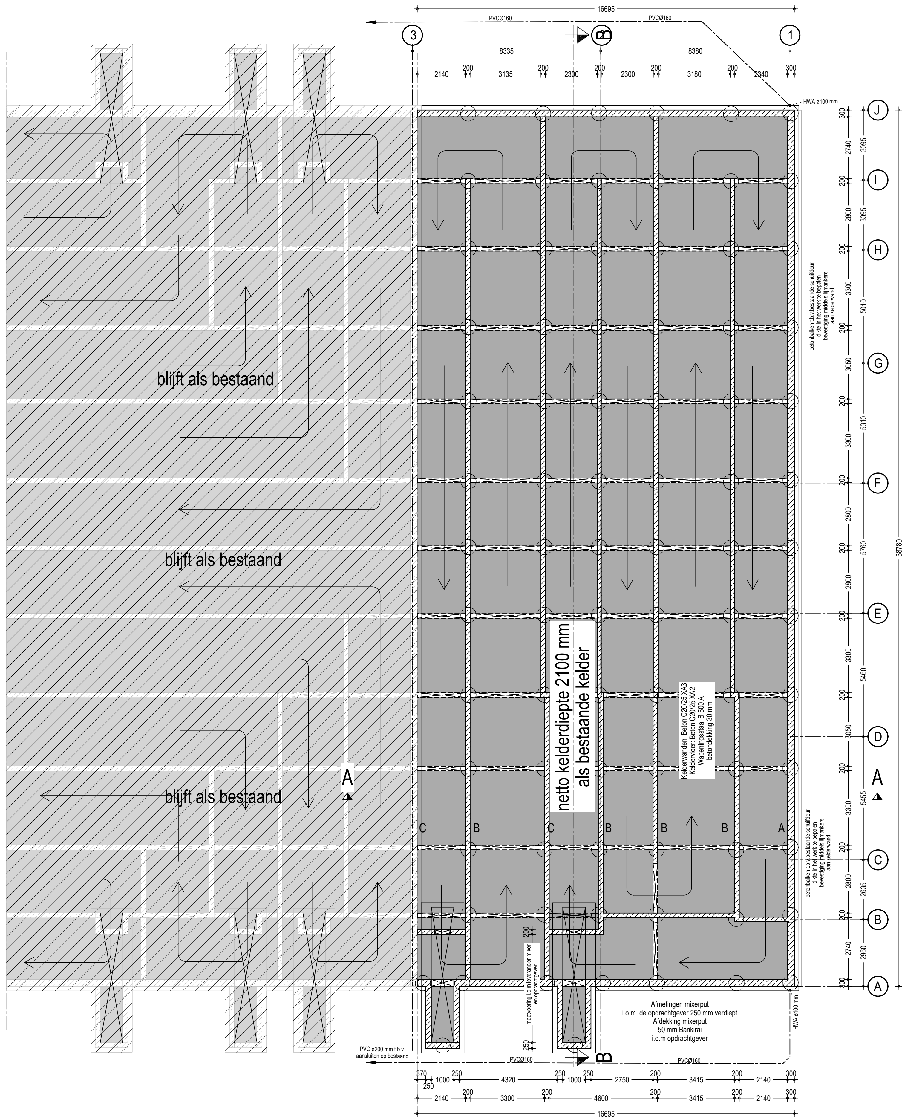
Kelderplan
