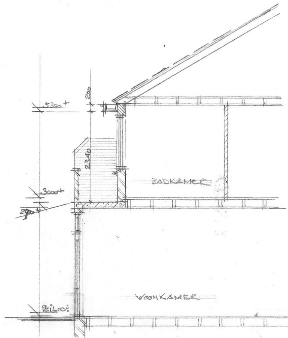
— DOORSNED E
