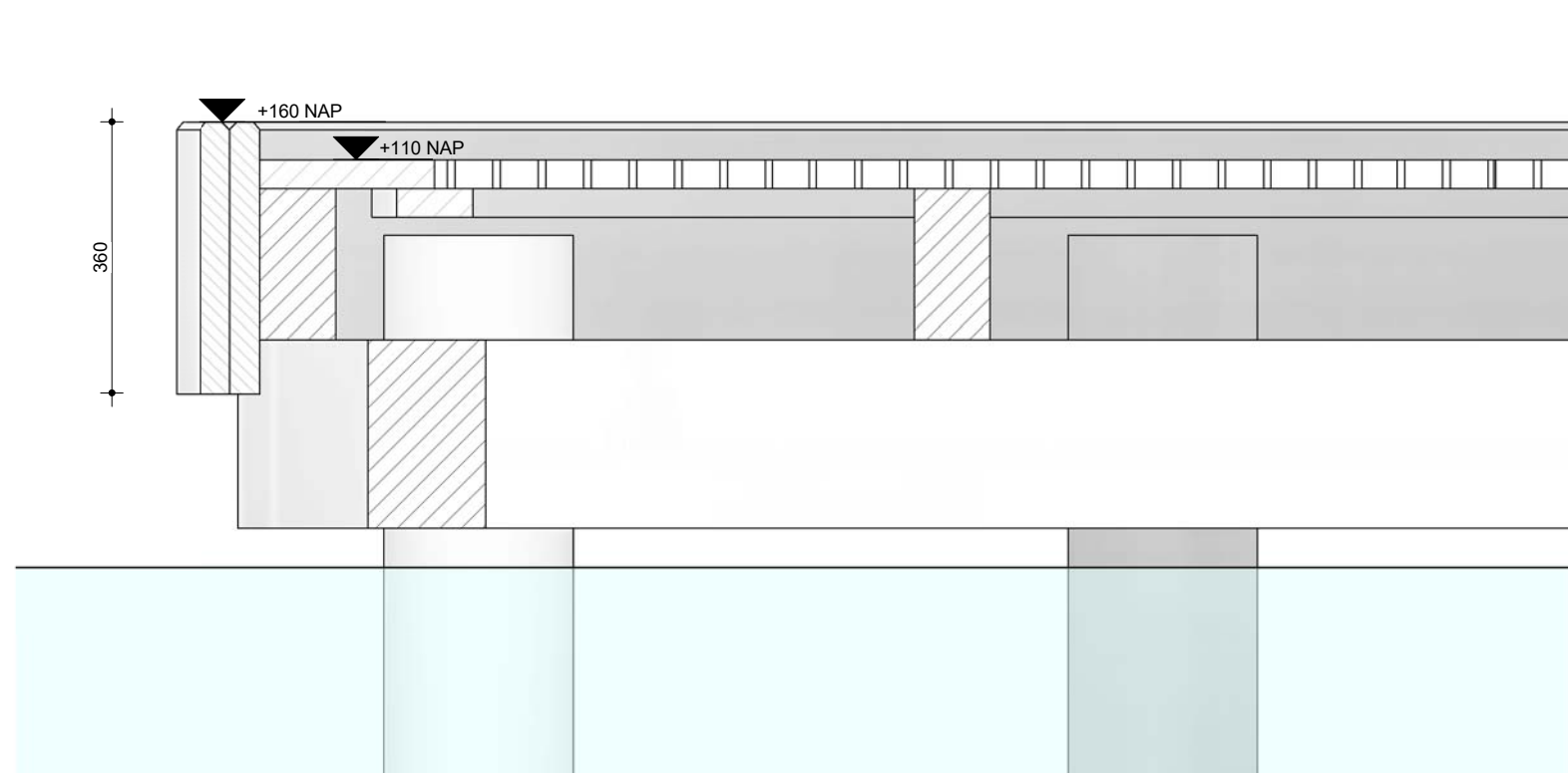
Detail waterterrassen
