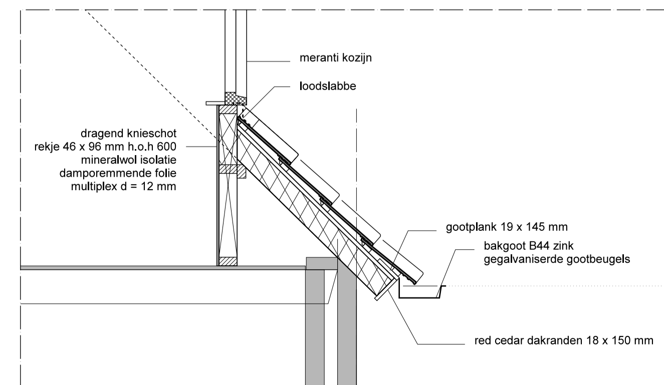
DETAIL 1
