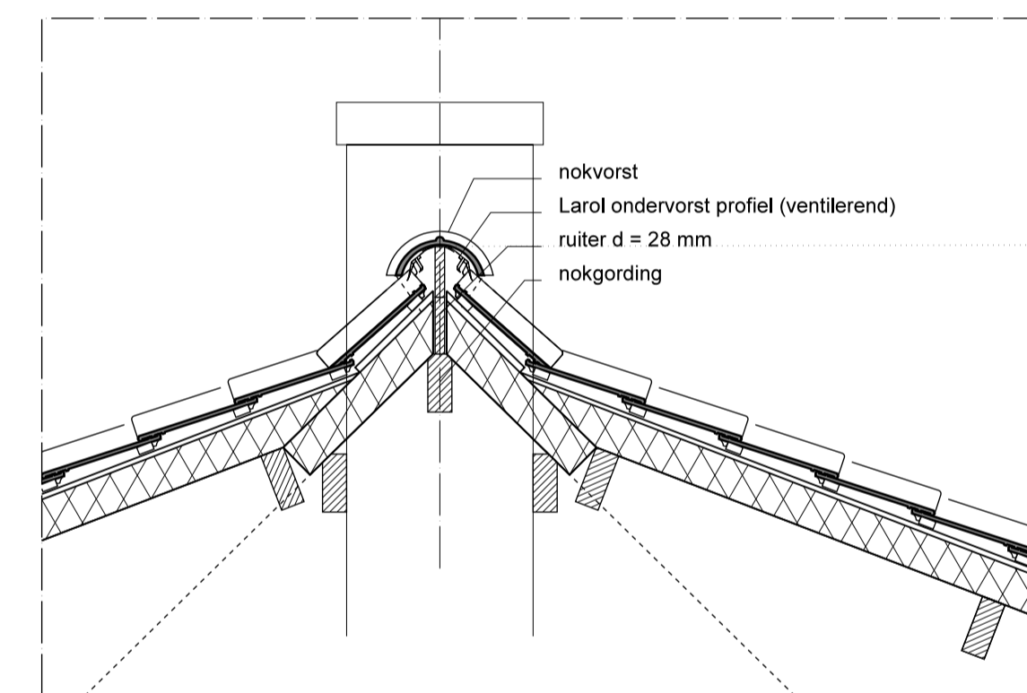
DETAIL 3
