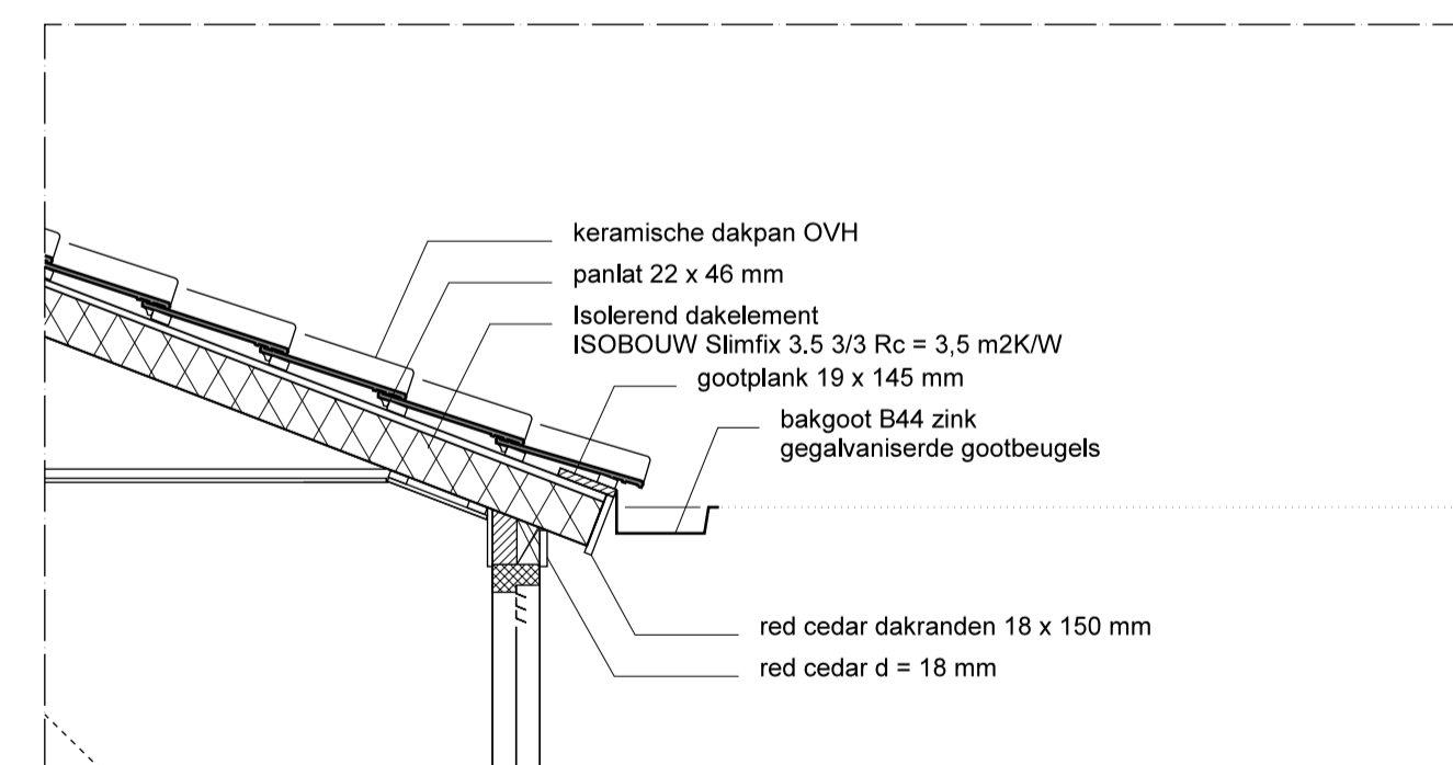
DETAIL 2
