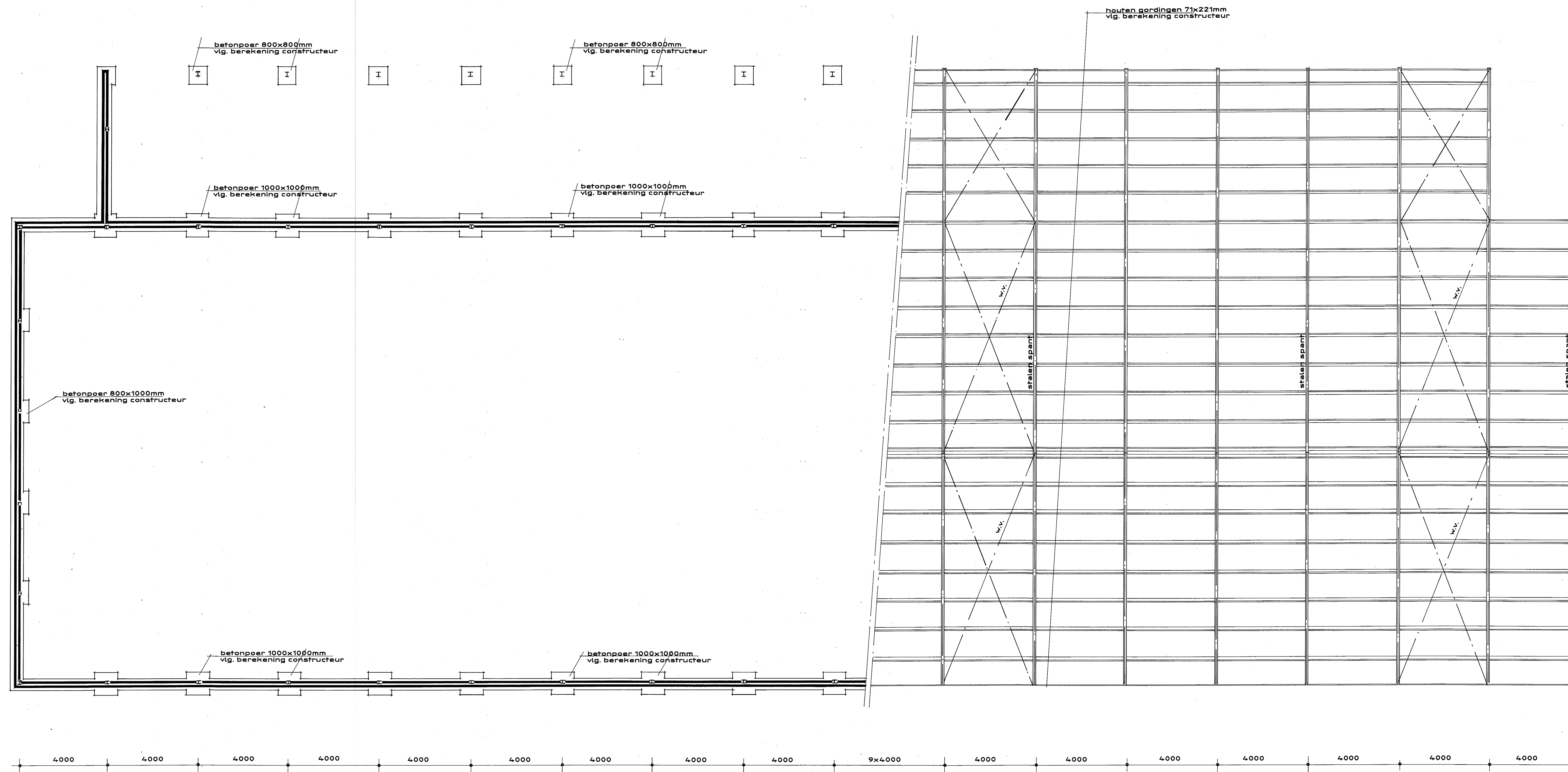
fundering - riolering
