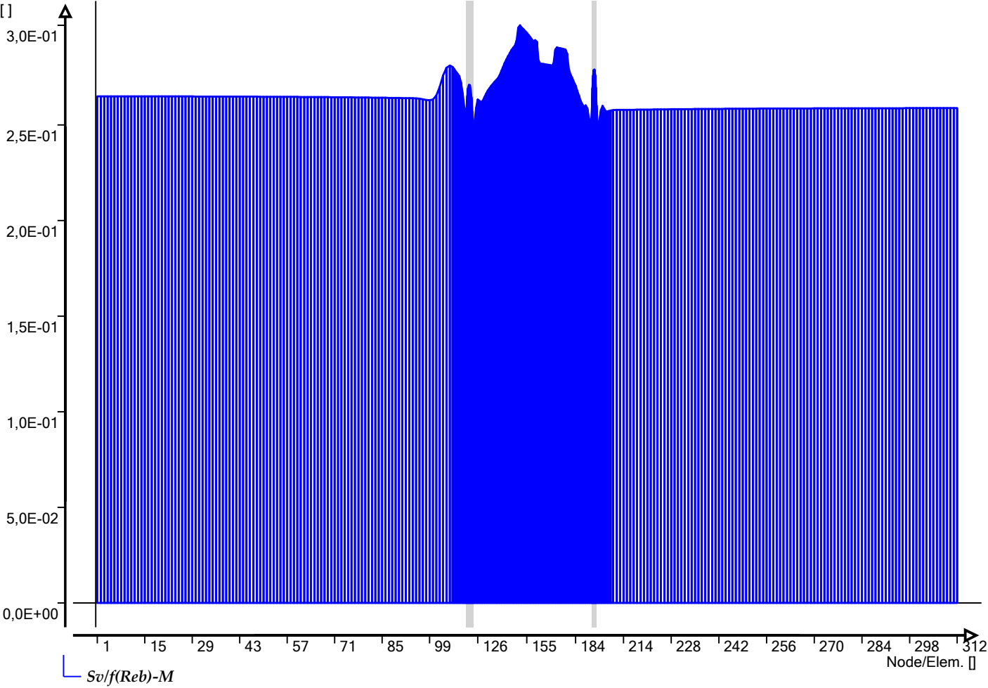
Graphs of table 'NEN3650 maximum unit check stresses' Ple4Win: BC4, PPS DN200 resreve leiding t = 6.35 mm
