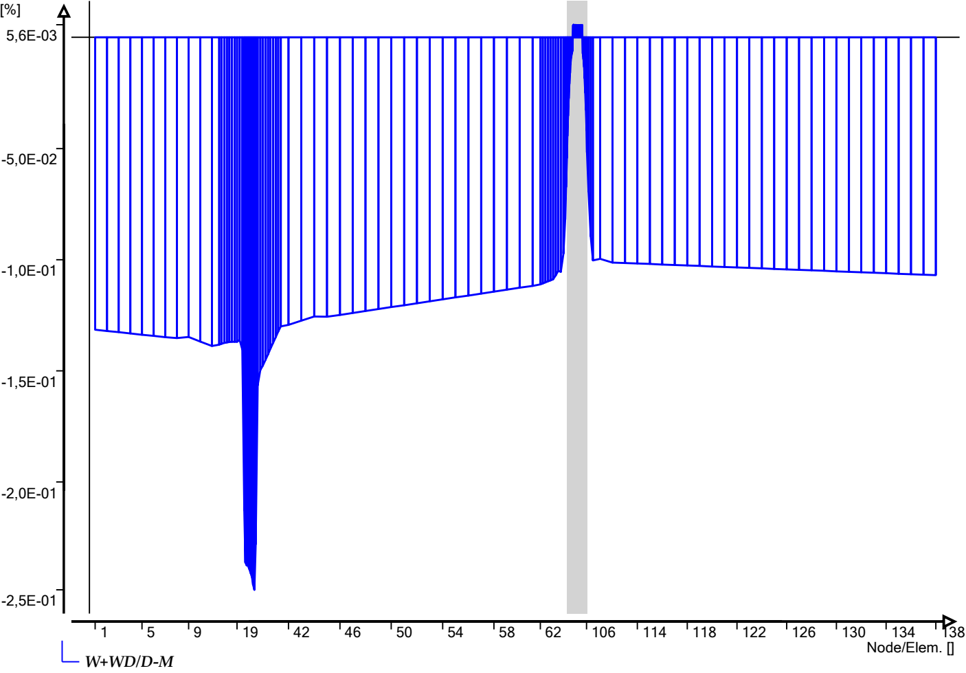
Graphs of table 'Maximum radial deformations (NEN ... Ple4Win: Air liquide, DN250 O2 leiding dijkvak 22, BC4
