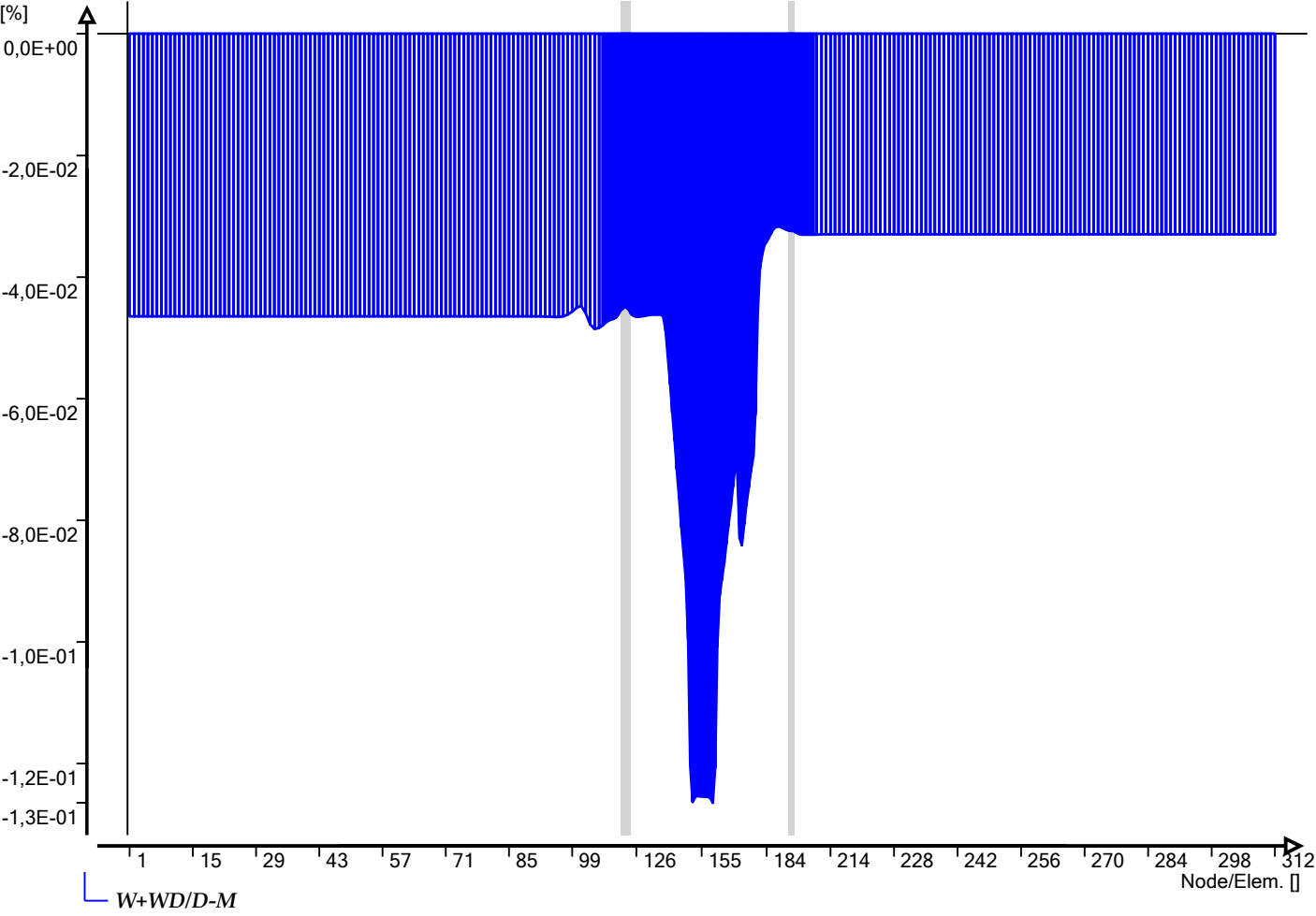
Graphs of table 'Maximum radial deformations (NEN 36... Ple4Win: BC3, PPS DN200 resreve leiding t = 6.35 mm
