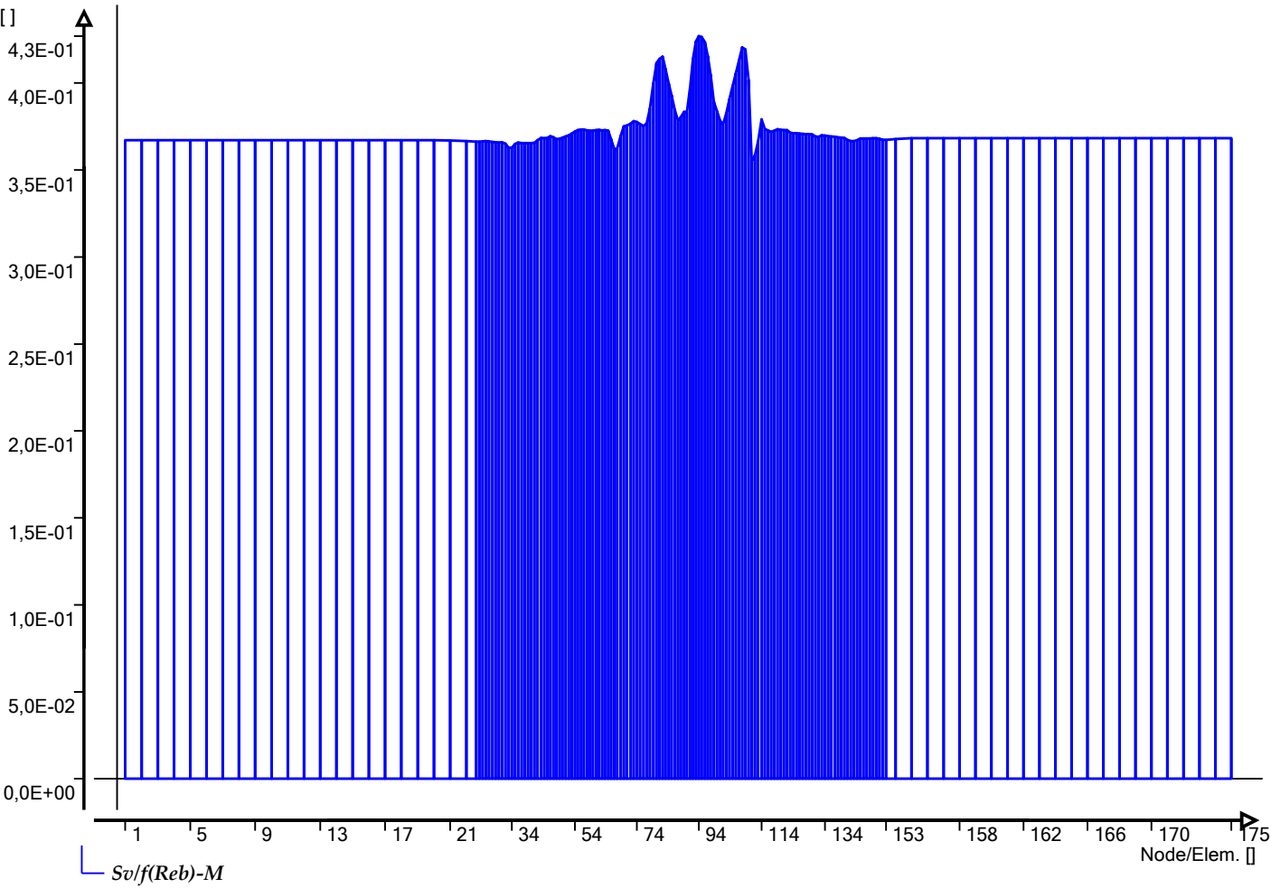
Graphs of table 'NEN3650 maximum unit check ... Ple4Win: Air liquide, DN 250 O2 leiding dijkvak 19 en 20, BC4
