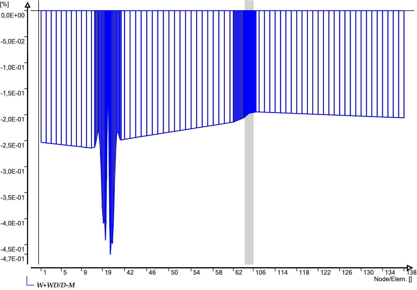
Graphs of table 'Maximum radial deformations (NEN ... Ple4Win: Air liquide, DN250 O2 leiding dijkvak 22, BC3
