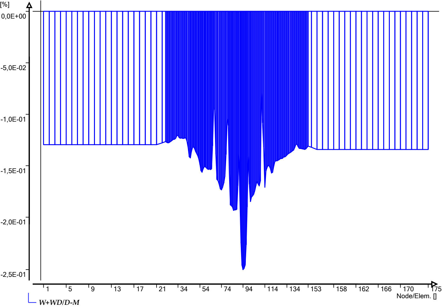
Graphs of table 'Maximum radial deformations ... Ple4Win: Air liquide, DN 250 O2 leiding dijkvak 19 en 20, BC4
