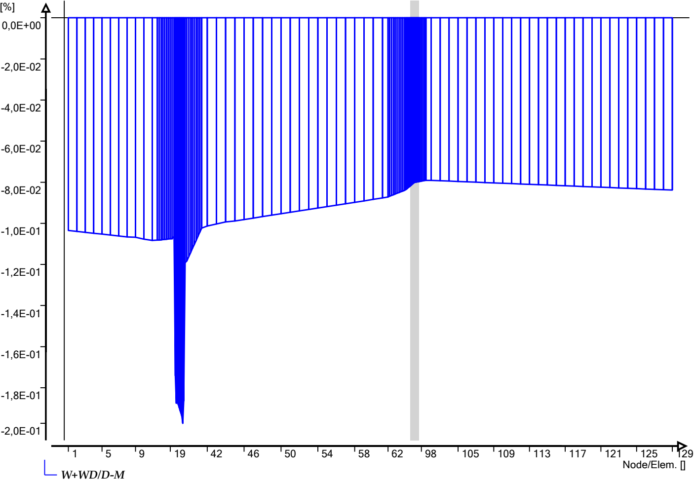
Graphs of table 'Maximum radial deformations (NEN ... Ple4Win: Air liquide, DN150 O2 leiding dijkvak 22, BC3
