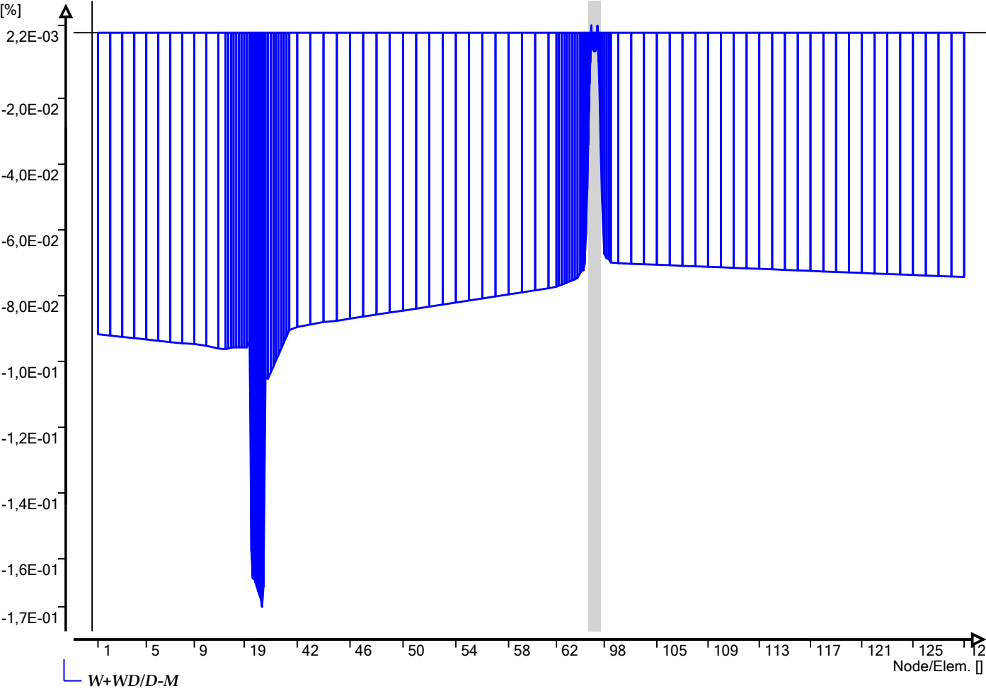
Graphs of table 'Maximum radial deformations (NEN ... Ple4Win: Air liquide, DN150 O2 leiding dijkvak 22, BC4
