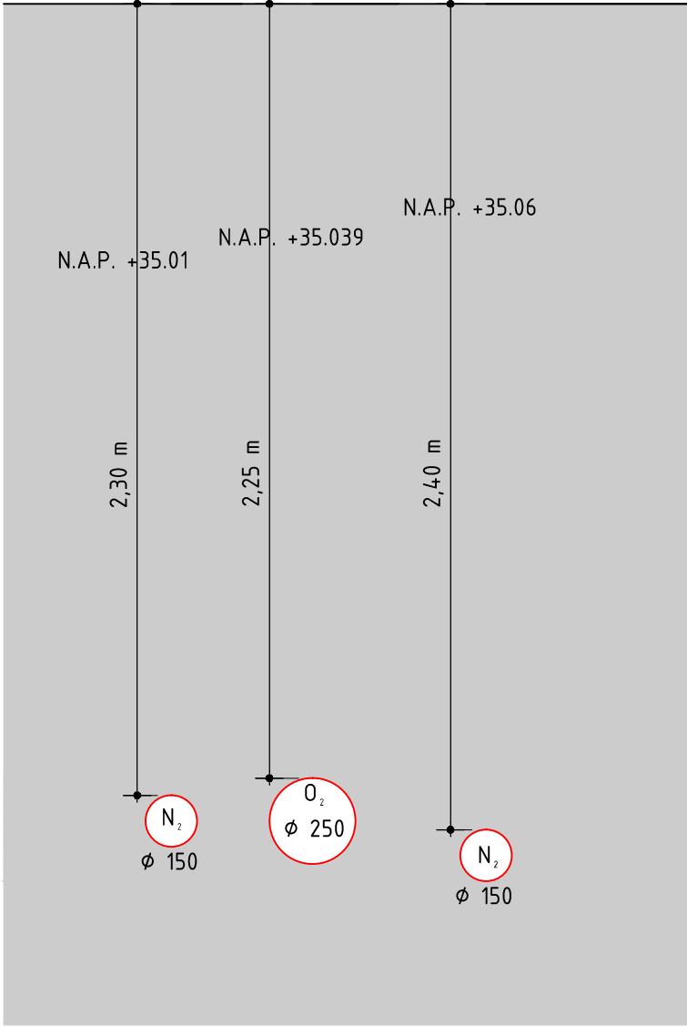
DWARSDOORSNEDE C - C'
