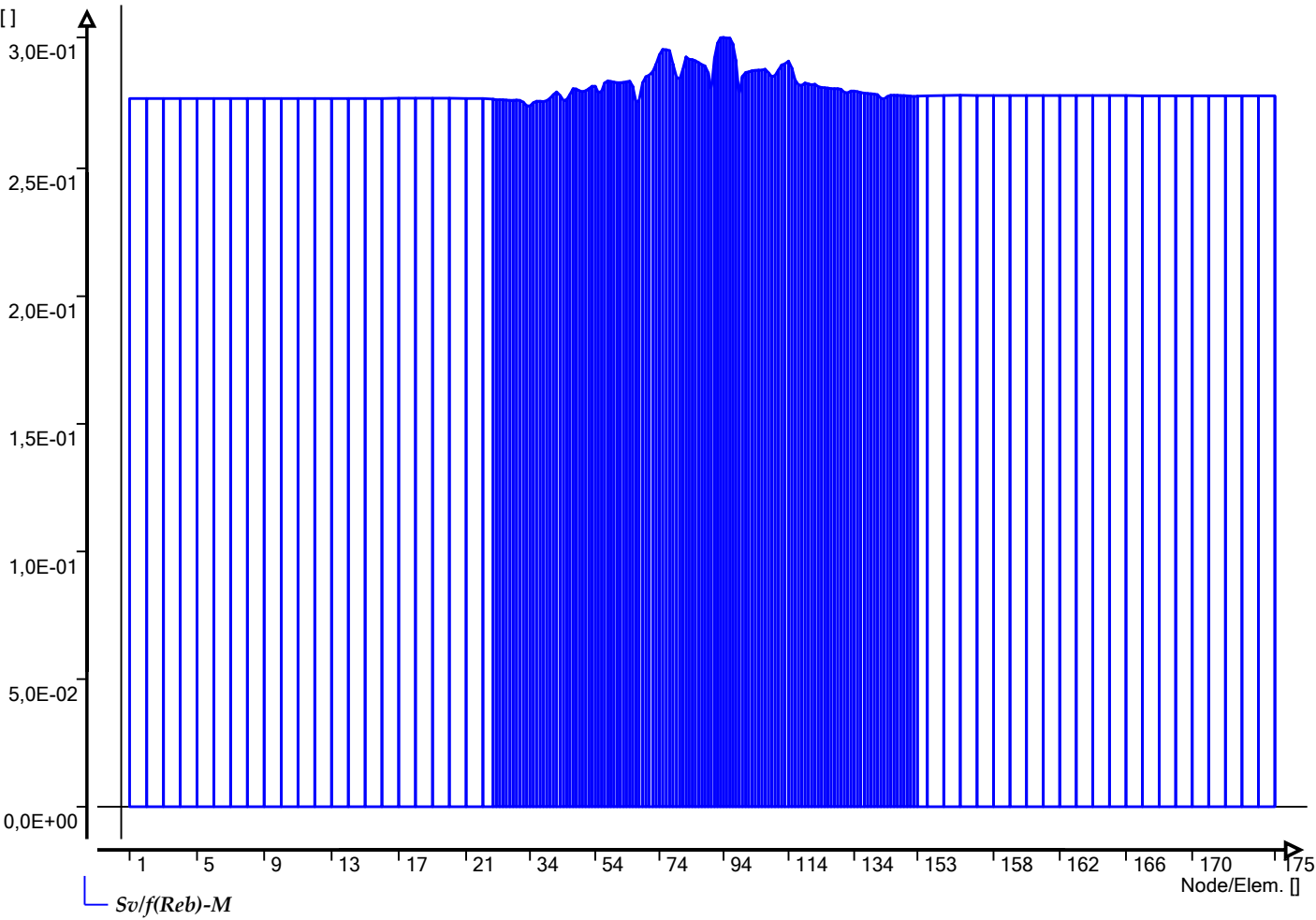
Graphs of table 'NEN3650 maximum unit check ... Ple4Win: Air liquide, DN 150 O2 leiding dijkvak 19 en 20, BC4
