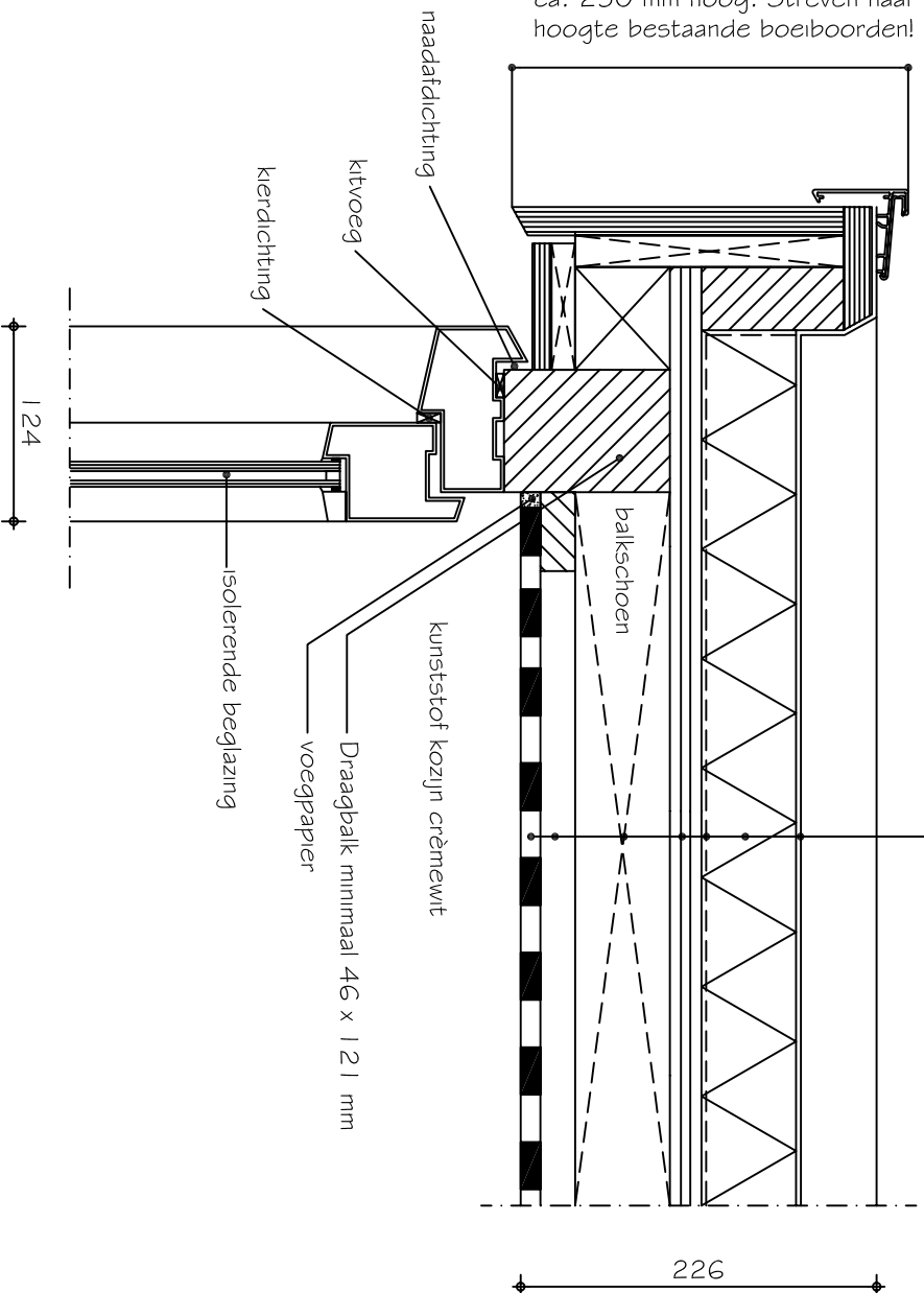
Principedetail 3 schaal 1:5 (bron: SBR 2017)
