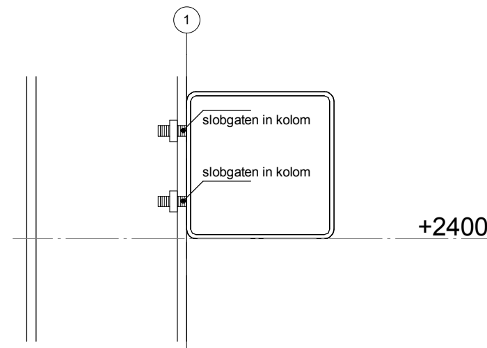
Detail 3 - 1:5
