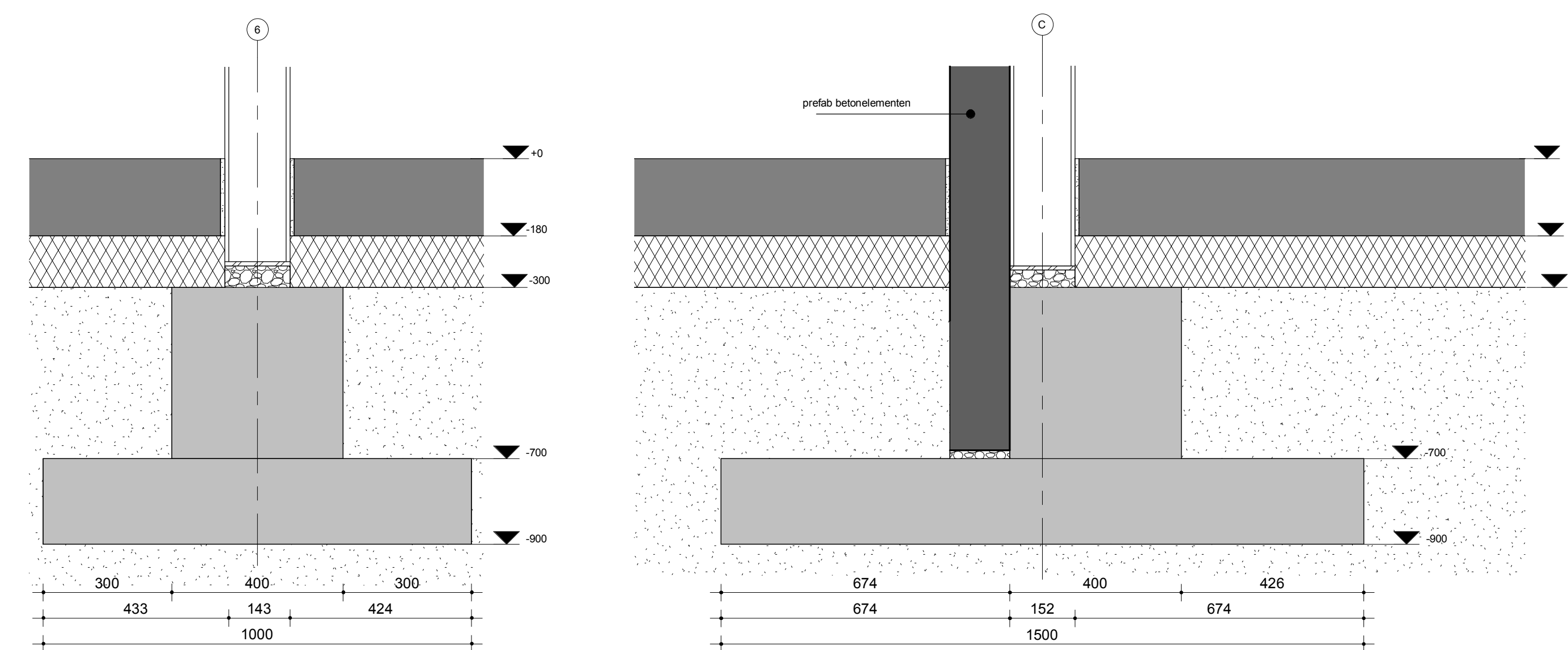
Detail F3
