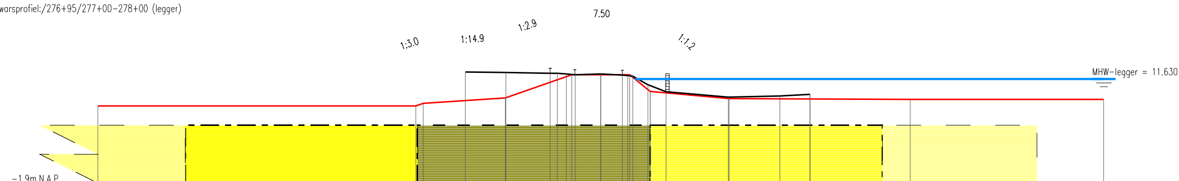
Dwarsprofiel: /276+95/277+00-278+00 (legger)
