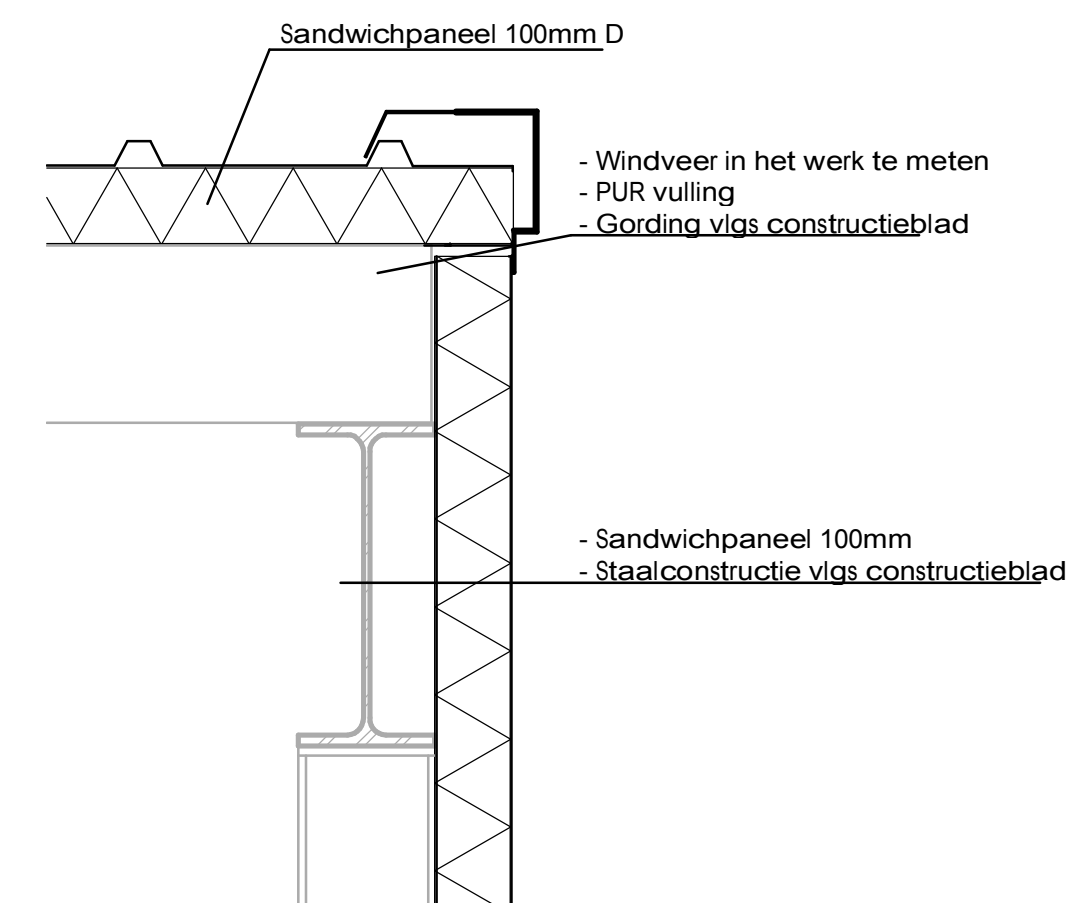
DETAIL G 1:10
