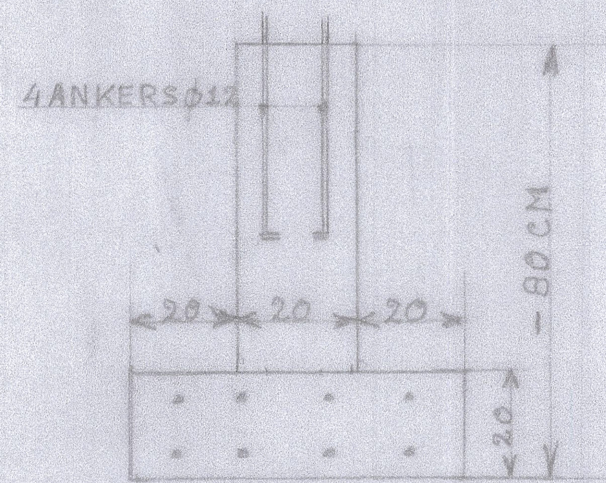
FUNDERING
