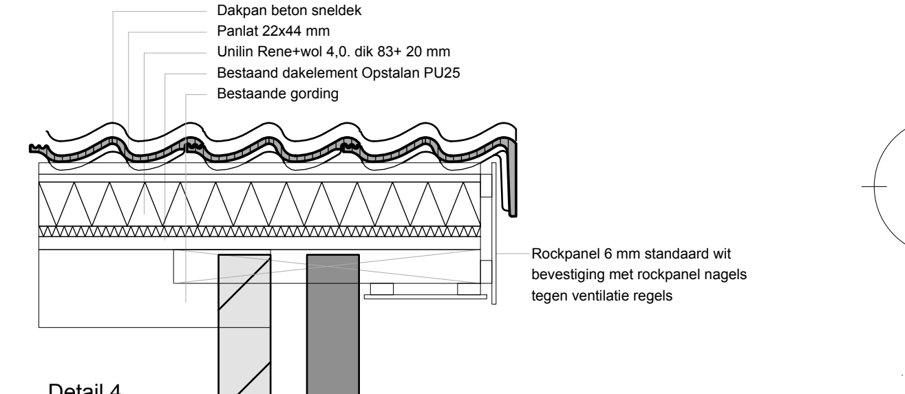
Detail 4
