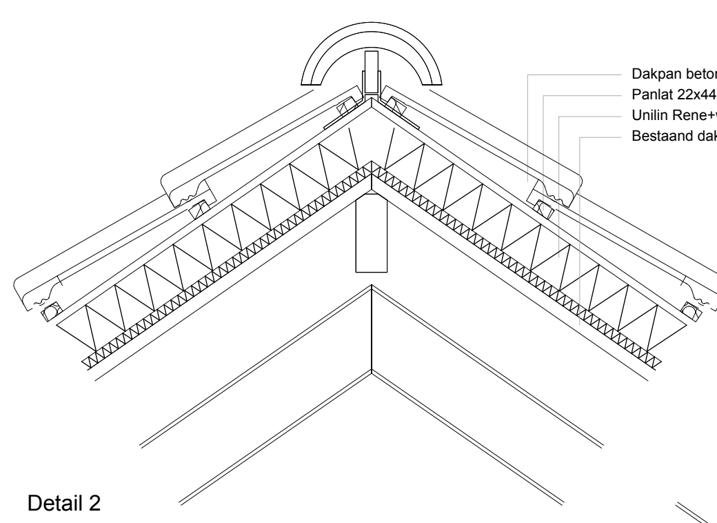
Detail 2
