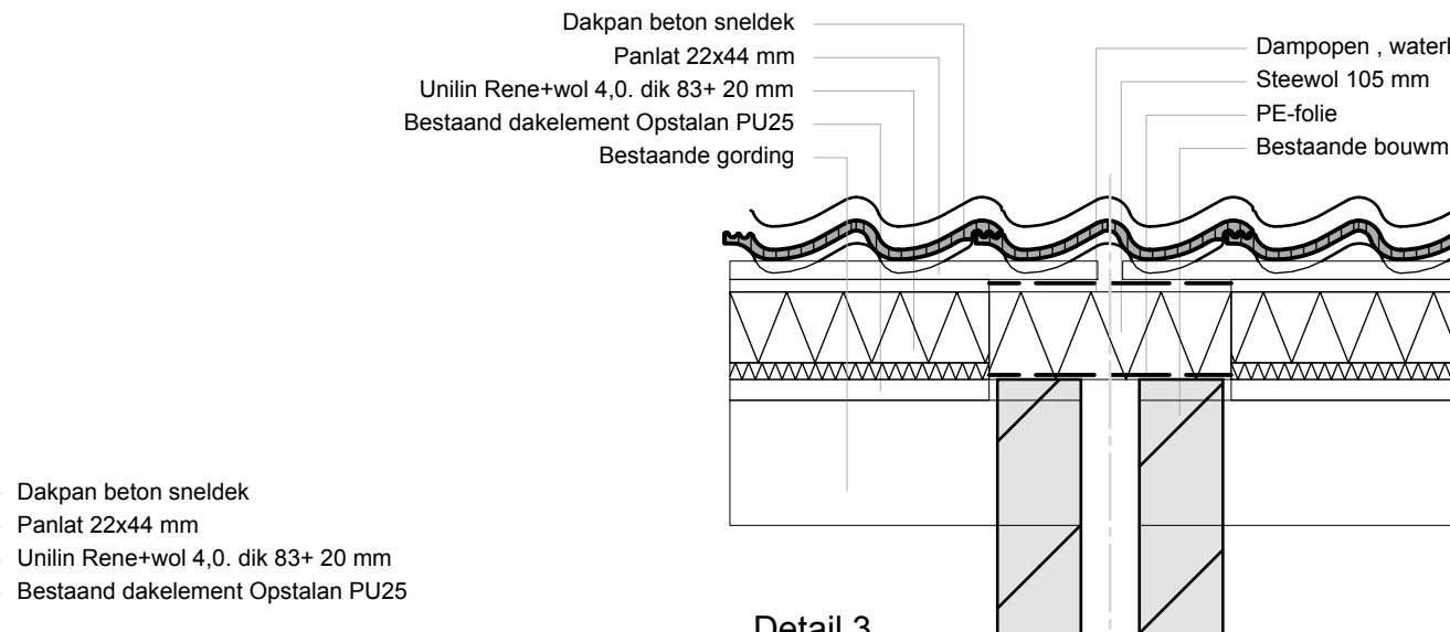
Detail 3
