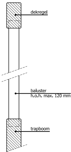
trapleuning
