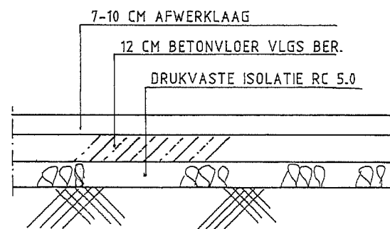
DETAIL 3
