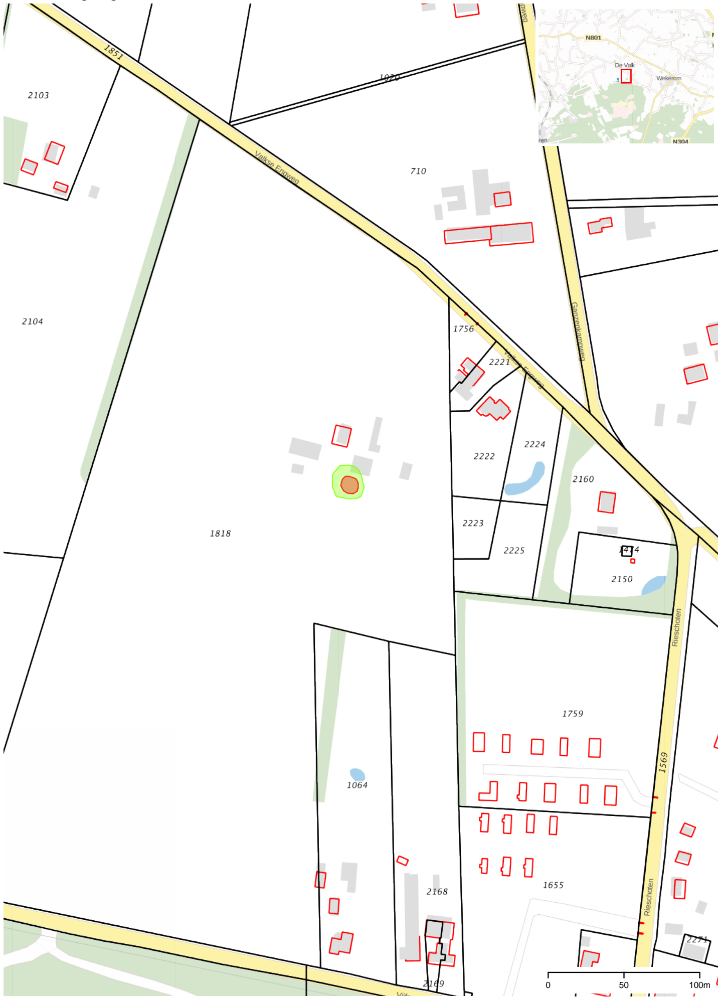
I-contour zink grondwater
