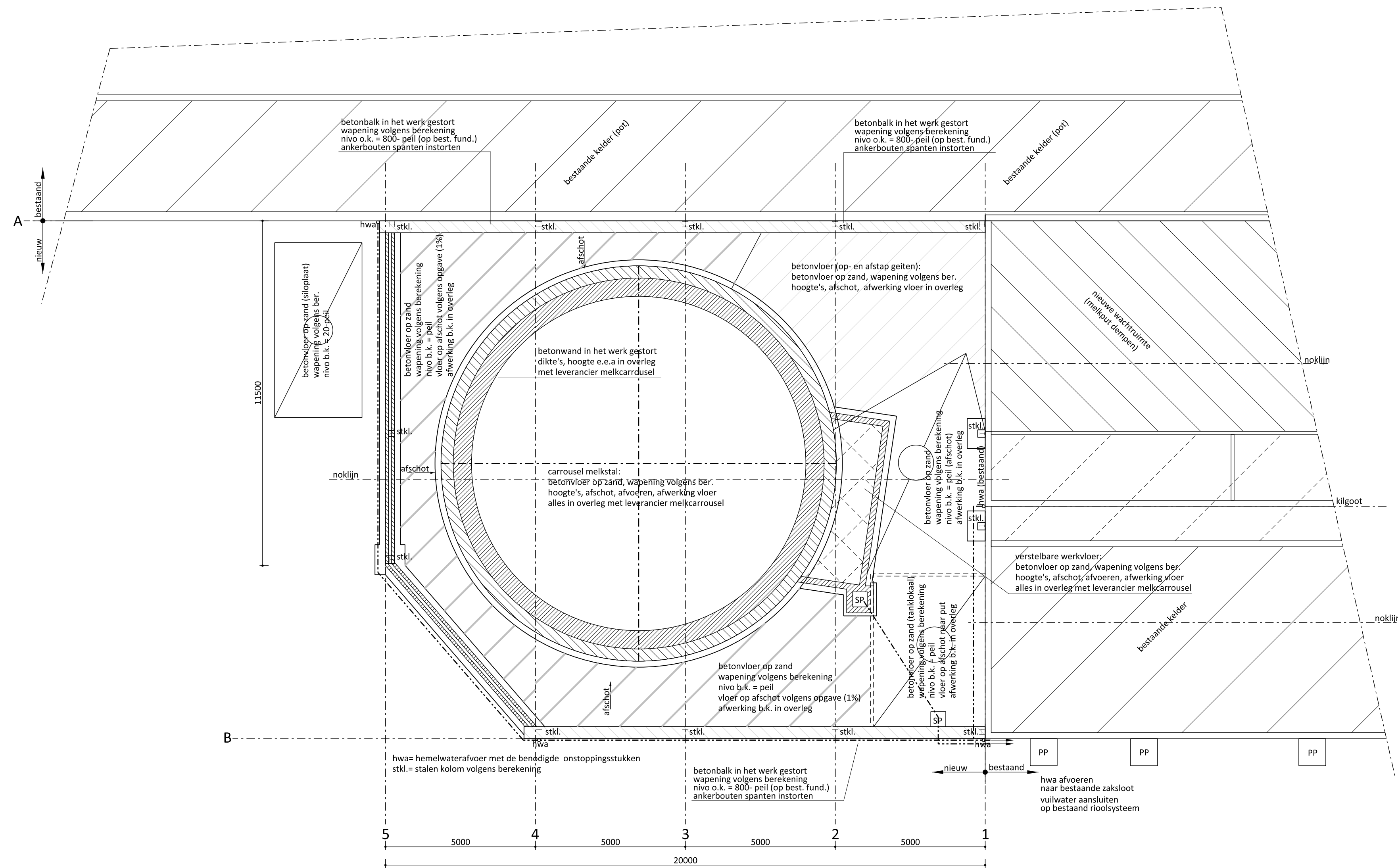
Funderingsplan
