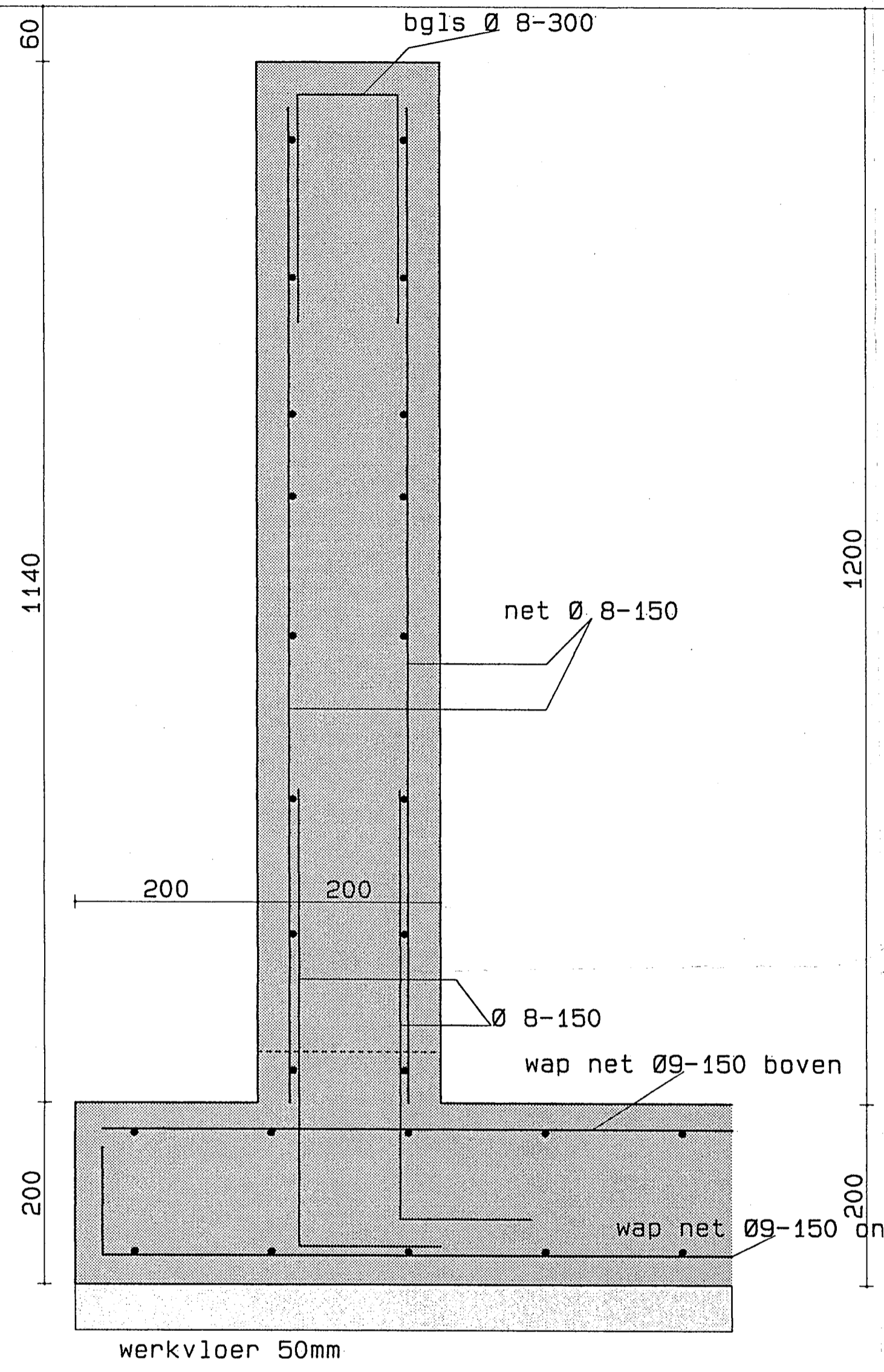
detail tpv laadkuil/wand
