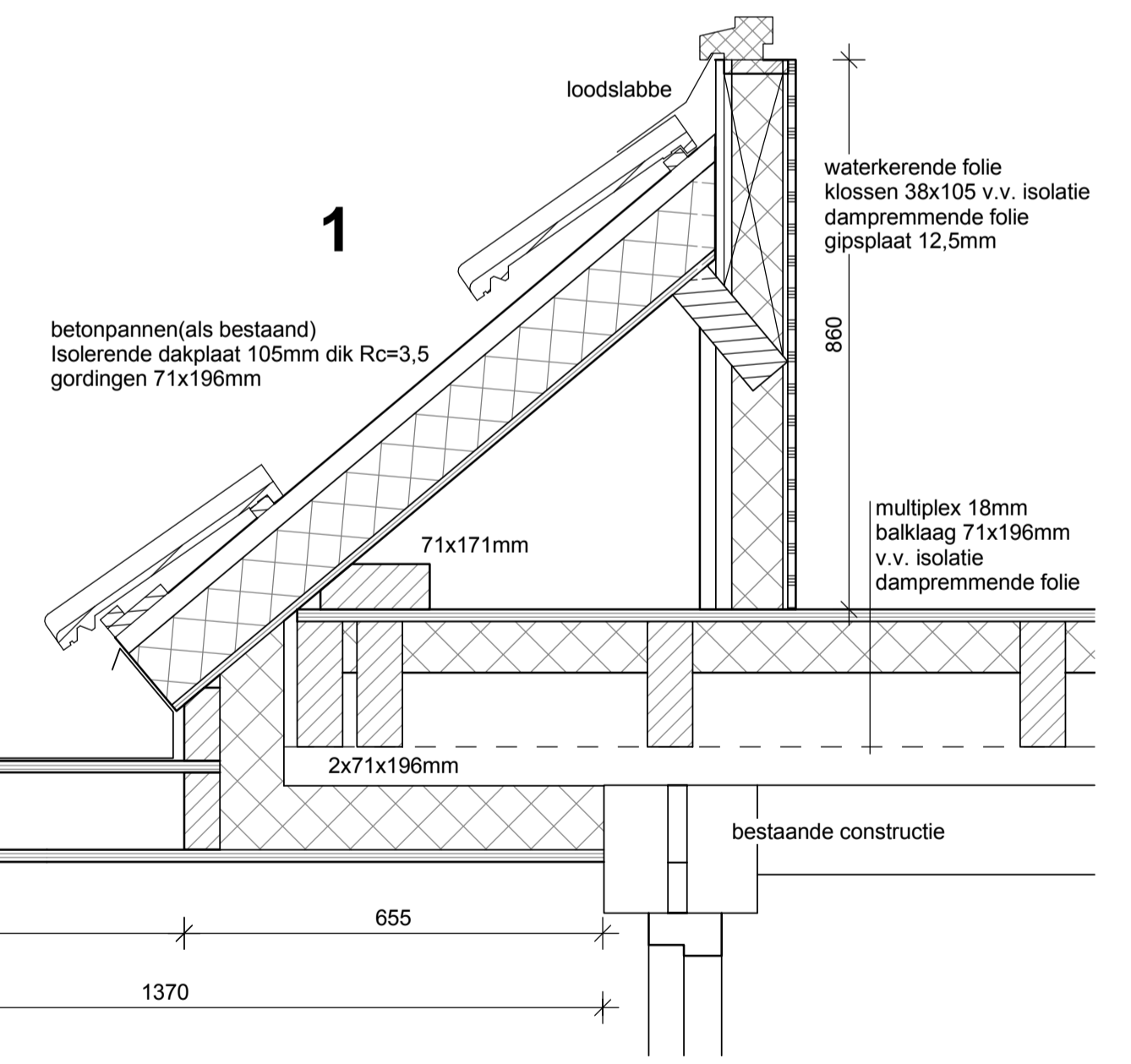
Principedetails Schaal 1:10
